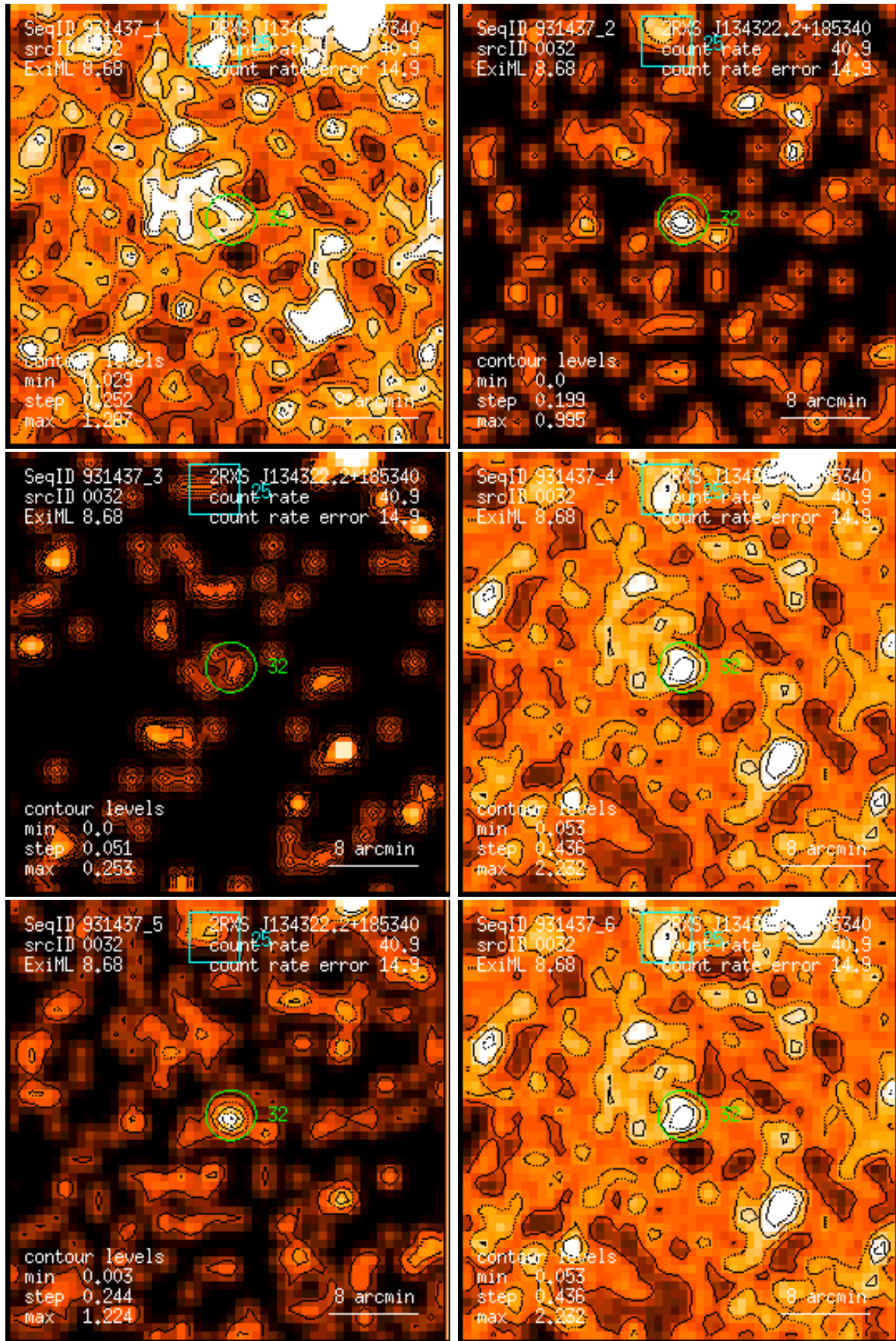
Figure 32: RASS 931437: detection 0032: band rate images, Gaussian filter: (1) PSPC channels 11 – 41, (2) 52 – 90, (3) 91 – 201, (4) 11 – 235, (5) 52 – 201, (6) 11 – 201. Broad band rates in counts/ks. Band rate contour levels in counts/ks/arcmin 2 .
