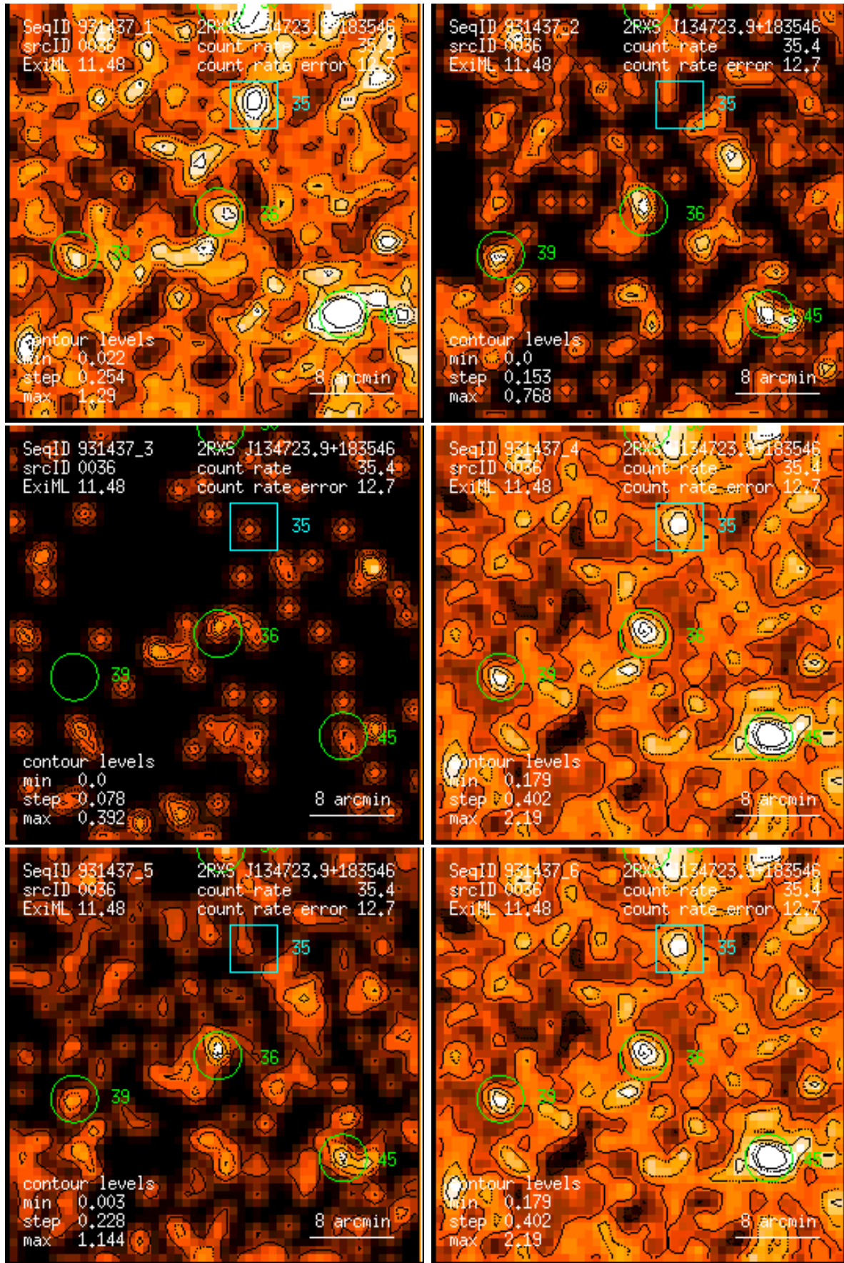
Figure 36: RASS 931437: detection 0036: band rate images, Gaussian filter: (1) PSPC channels 11 – 41, (2) 52 – 90, (3) 91 – 201, (4) 11 – 235, (5) 52 – 201, (6) 11 – 201. Broad band rates in counts/ks. Band rate contour levels in counts/ks/arcmin 2 .
