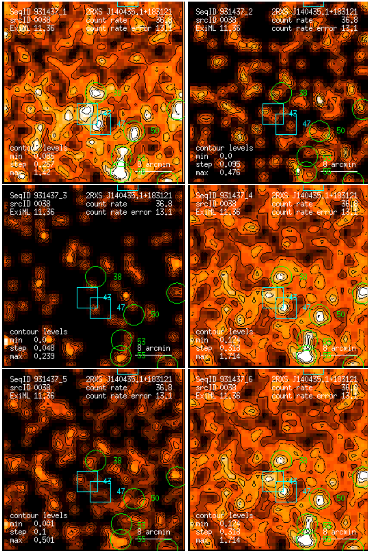
Figure 38: RASS 931437: detection 0038: band rate images, Gaussian filter: (1) PSPC channels 11 – 41, (2) 52 – 90, (3) 91 – 201, (4) 11 – 235, (5) 52 – 201, (6) 11 – 201. Broad band rates in counts/ks. Band rate contour levels in counts/ks/arcmin 2 .
