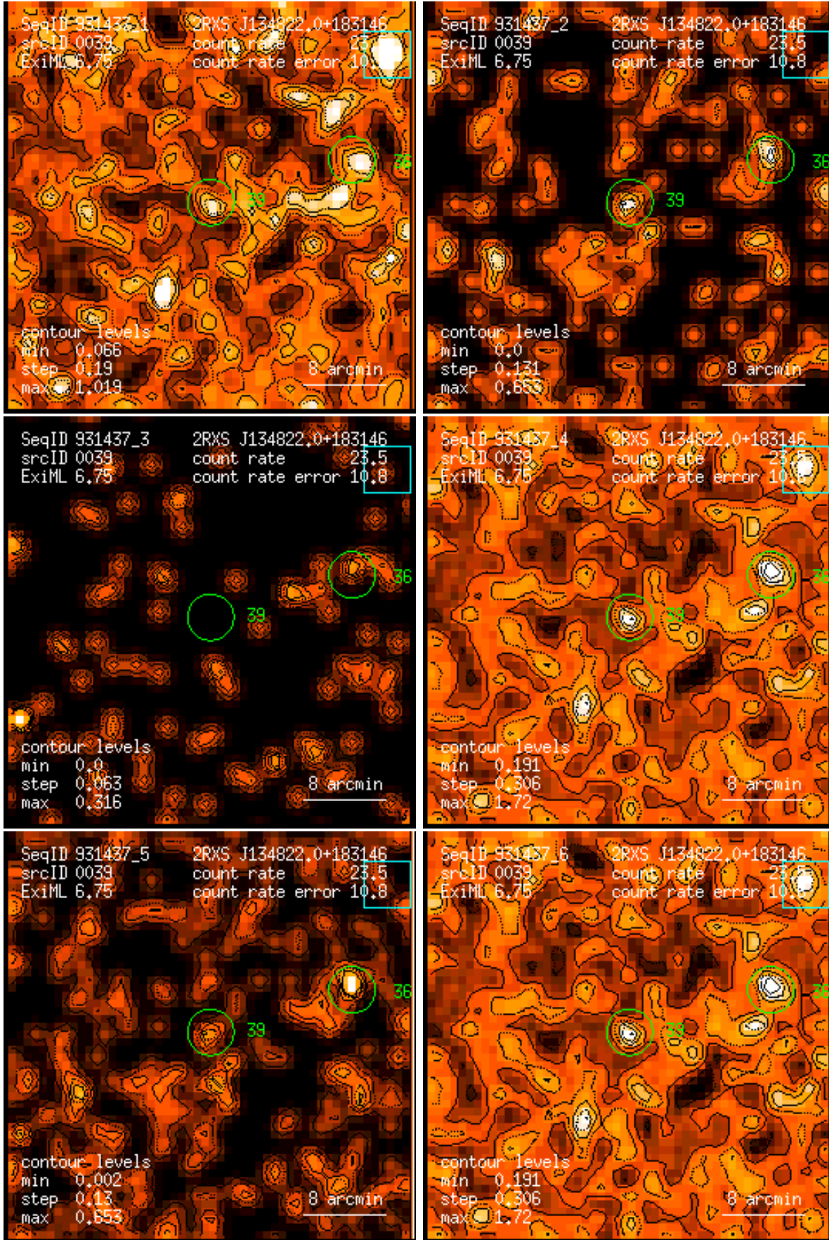
Figure 39: RASS 931437: detection 0039: band rate images, Gaussian filter: (1) PSPC channels 11 – 41, (2) 52 – 90, (3) 91 – 201, (4) 11 – 235, (5) 52 – 201, (6) 11 – 201. Broad band rates in counts/ks. Band rate contour levels in counts/ks/arcmin 2 .
