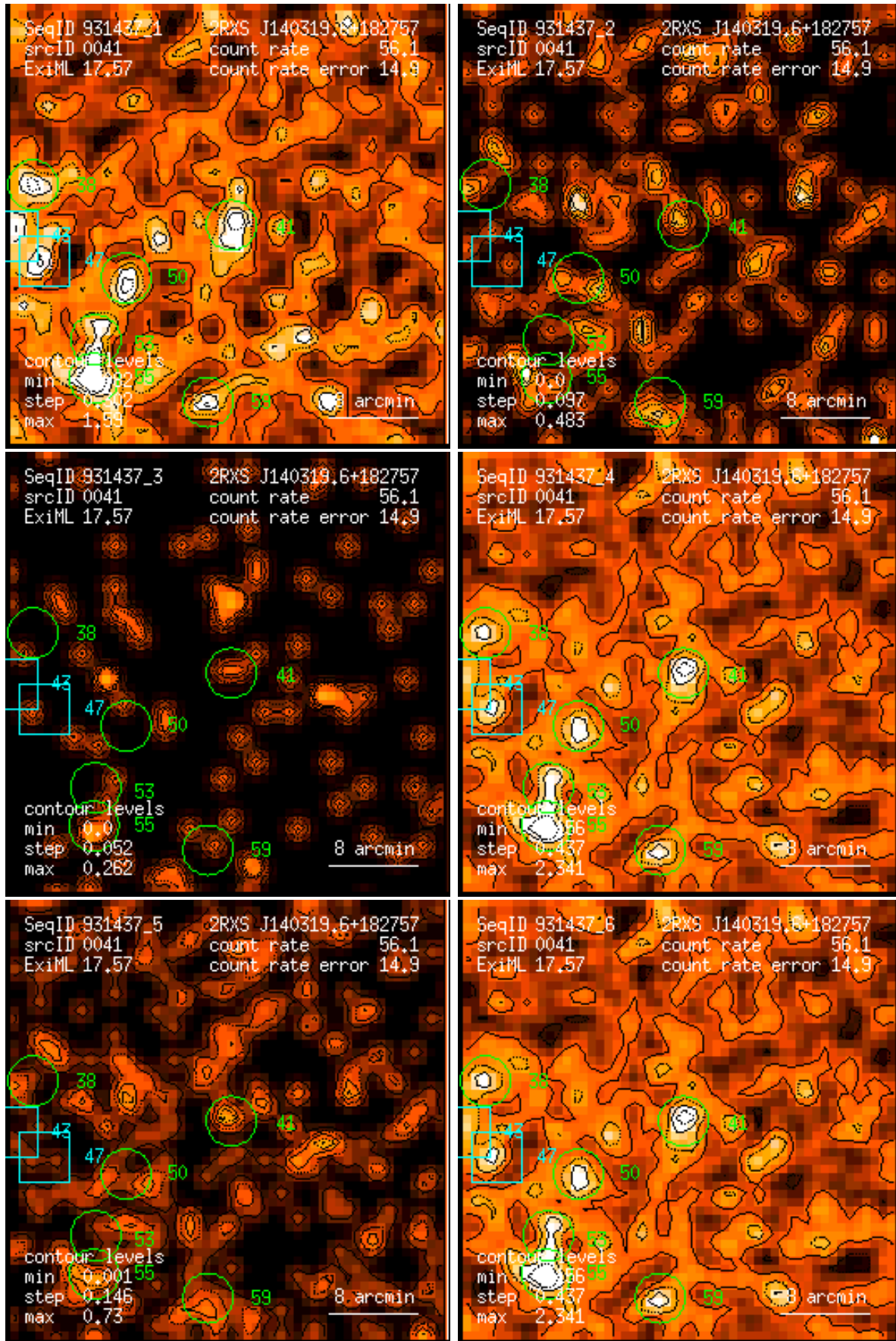
Figure 41: RASS 931437: detection 0041: band rate images, Gaussian filter: (1) PSPC channels 11 – 41, (2) 52 – 90, (3) 91 – 201, (4) 11 – 235, (5) 52 – 201, (6) 11 – 201. Broad band rates in counts/ks. Band rate contour levels in counts/ks/arcmin 2 .
