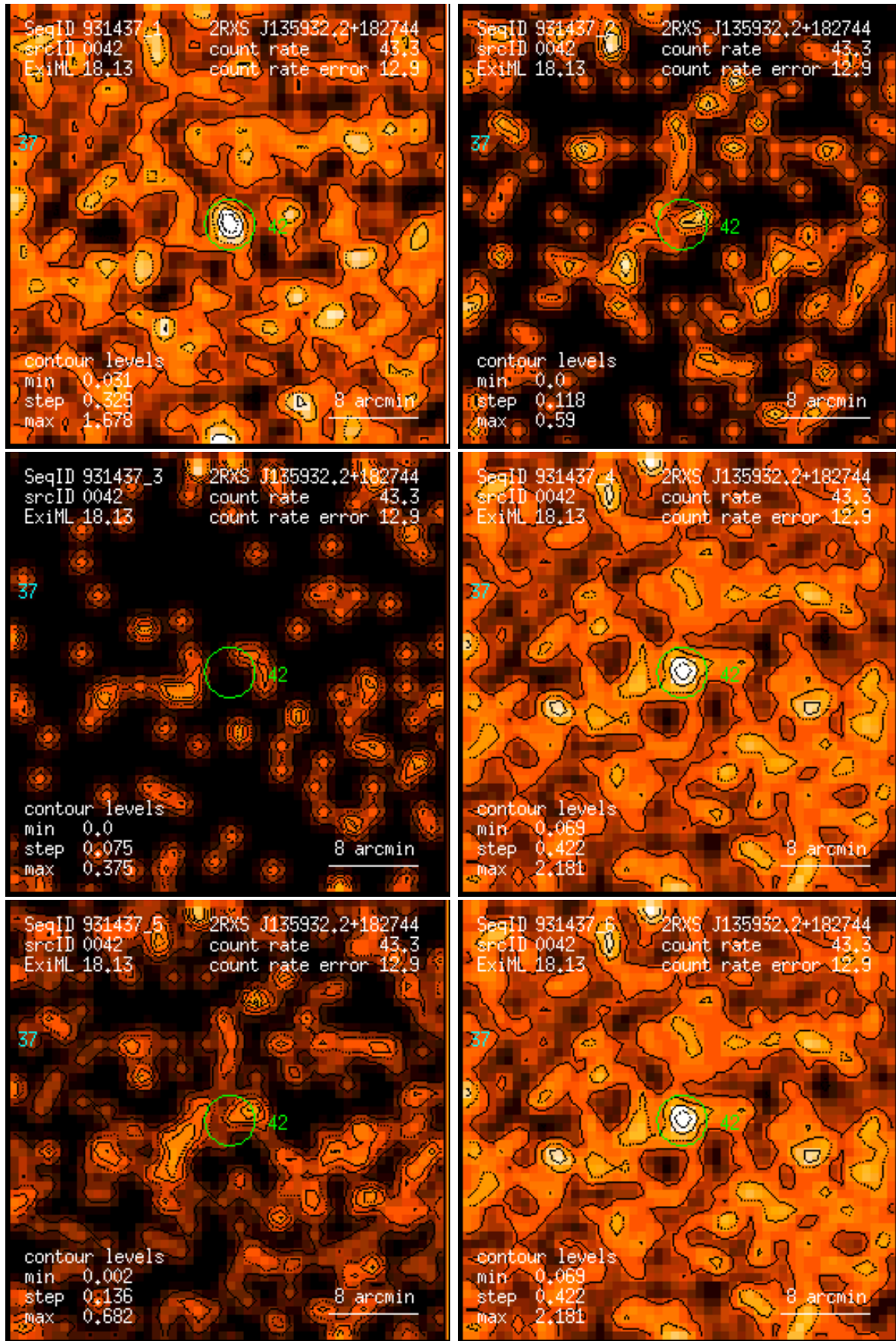
Figure 42: RASS 931437: detection 0042: band rate images, Gaussian filter: (1) PSPC channels 11 – 41, (2) 52 – 90, (3) 91 – 201, (4) 11 – 235, (5) 52 – 201, (6) 11 – 201. Broad band rates in counts/ks. Band rate contour levels in counts/ks/arcmin 2 .
