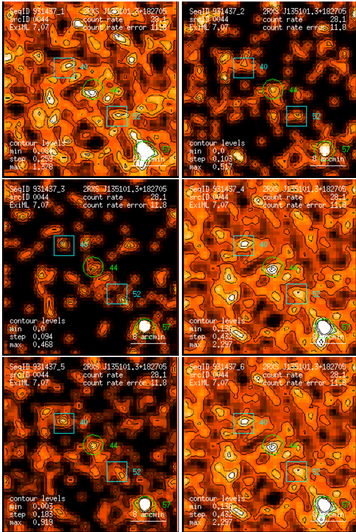
Figure 44: RASS 931437: detection 0044: band rate images, Gaussian filter: (1) PSPC channels 11 – 41, (2) 52 – 90, (3) 91 – 201, (4) 11 – 235, (5) 52 – 201, (6) 11 – 201. Broad band rates in counts/ks. Band rate contour levels in counts/ks/arcmin 2 .
