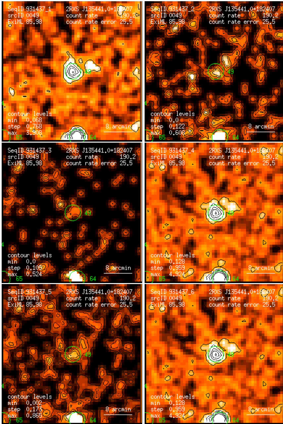
Figure 49: RASS 931437: detection 0049: band rate images, Gaussian filter: (1) PSPC channels 11 – 41, (2) 52 – 90, (3) 91 – 201, (4) 11 – 235, (5) 52 – 201, (6) 11 – 201. Broad band rates in counts/ks. Band rate contour levels in counts/ks/arcmin 2 .
