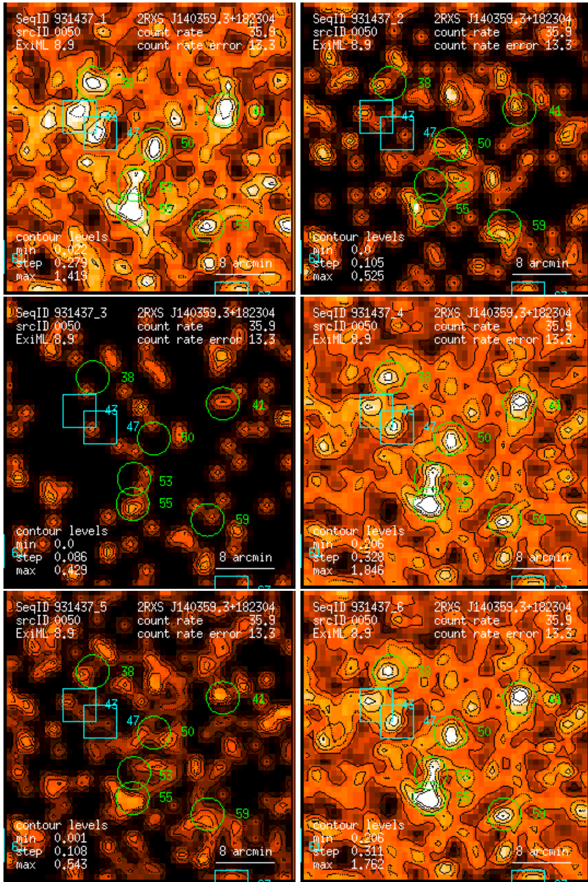
Figure 50: RASS 931437: detection 0050: band rate images, Gaussian filter: (1) PSPC channels 11 – 41, (2) 52 – 90, (3) 91 – 201, (4) 11 – 235, (5) 52 – 201, (6) 11 – 201. Broad band rates in counts/ks. Band rate contour levels in counts/ks/arcmin 2 .
