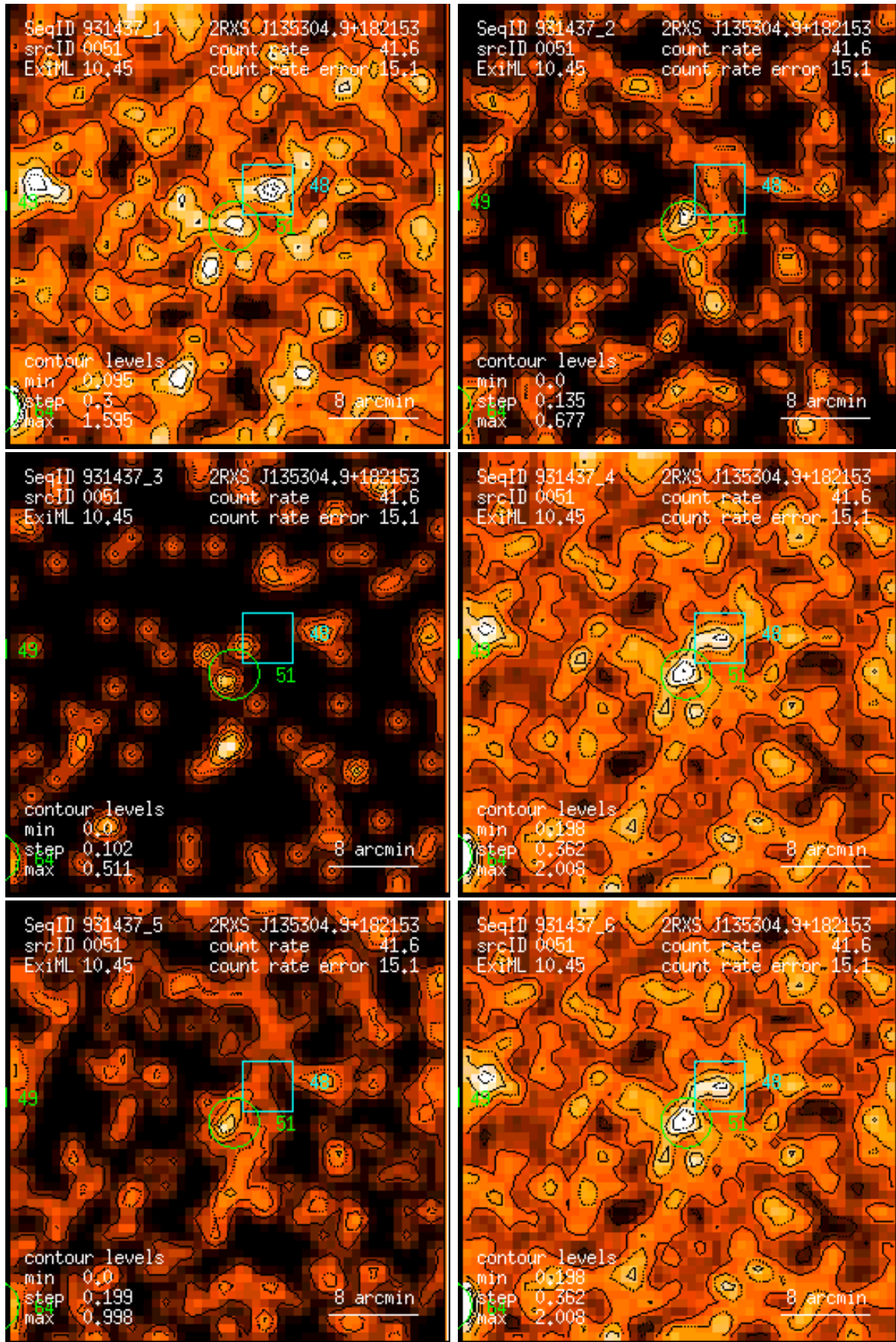
Figure 51: RASS 931437: detection 0051: band rate images, Gaussian filter: (1) PSPC channels 11 – 41, (2) 52 – 90, (3) 91 – 201, (4) 11 – 235, (5) 52 – 201, (6) 11 – 201. Broad band rates in counts/ks. Band rate contour levels in counts/ks/arcmin 2 .
