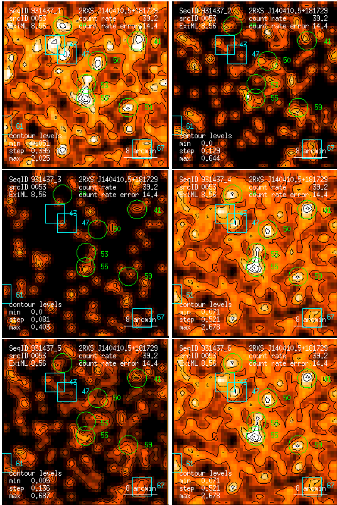
Figure 53: RASS 931437: detection 0053: band rate images, Gaussian filter: (1) PSPC channels 11 – 41, (2) 52 – 90, (3) 91 – 201, (4) 11 – 235, (5) 52 – 201, (6) 11 – 201. Broad band rates in counts/ks. Band rate contour levels in counts/ks/arcmin 2 .
