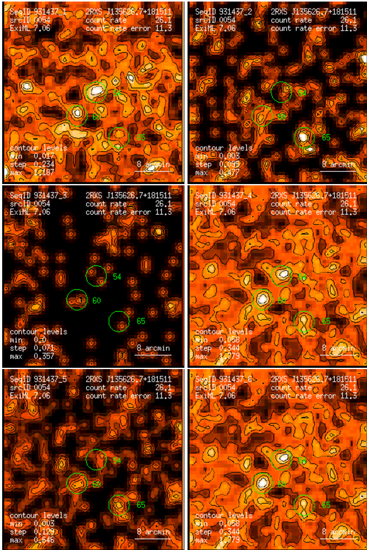
Figure 54: RASS 931437: detection 0054: band rate images, Gaussian filter: (1) PSPC channels 11 – 41, (2) 52 – 90, (3) 91 – 201, (4) 11 – 235, (5) 52 – 201, (6) 11 – 201. Broad band rates in counts/ks. Band rate contour levels in counts/ks/arcmin 2 .
