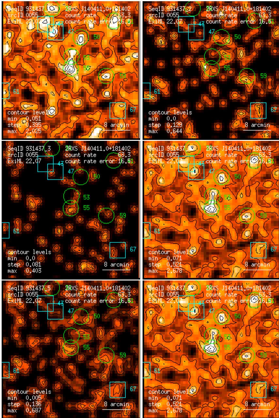
Figure 55: RASS 931437: detection 0055: band rate images, Gaussian filter: (1) PSPC channels 11 – 41, (2) 52 – 90, (3) 91 – 201, (4) 11 – 235, (5) 52 – 201, (6) 11 – 201. Broad band rates in counts/ks. Band rate contour levels in counts/ks/arcmin 2 .
