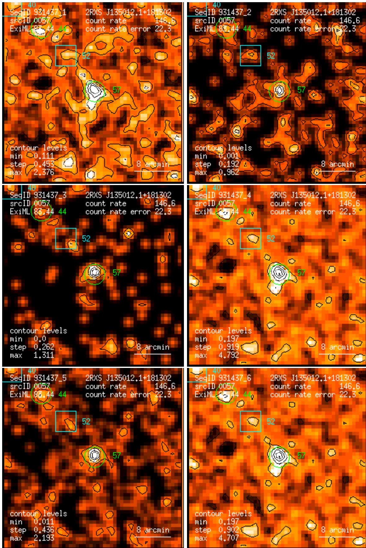
Figure 57: RASS 931437: detection 0057: band rate images, Gaussian filter: (1) PSPC channels 11 – 41, (2) 52 – 90, (3) 91 – 201, (4) 11 – 235, (5) 52 – 201, (6) 11 – 201. Broad band rates in counts/ks. Band rate contour levels in counts/ks/arcmin 2 .
