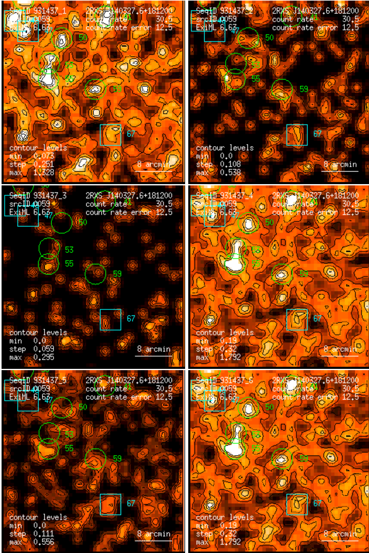
Figure 59: RASS 931437: detection 0059: band rate images, Gaussian filter: (1) PSPC channels 11 – 41, (2) 52 – 90, (3) 91 – 201, (4) 11 – 235, (5) 52 – 201, (6) 11 – 201. Broad band rates in counts/ks. Band rate contour levels in counts/ks/arcmin 2 .
