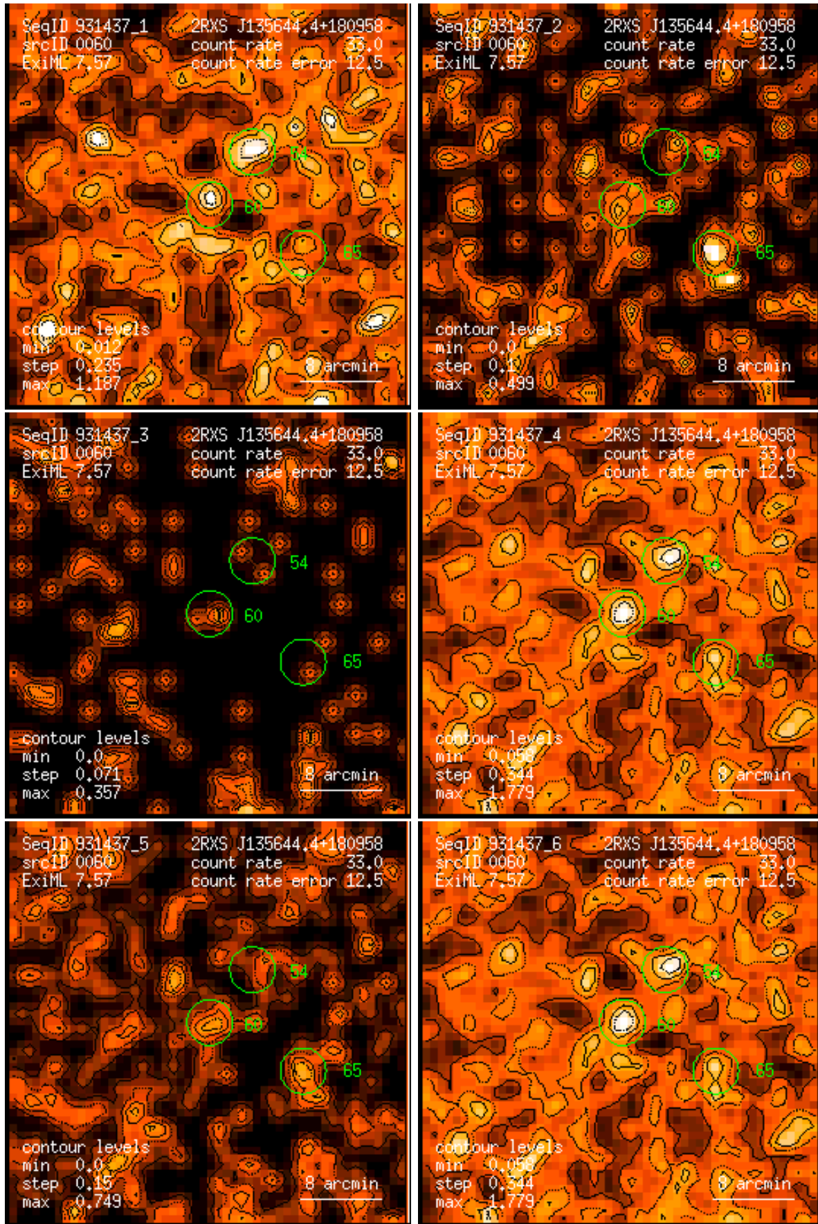
Figure 60: RASS 931437: detection 0060: band rate images, Gaussian filter: (1) PSPC channels 11 – 41, (2) 52 – 90, (3) 91 – 201, (4) 11 – 235, (5) 52 – 201, (6) 11 – 201. Broad band rates in counts/ks. Band rate contour levels in counts/ks/arcmin 2 .
