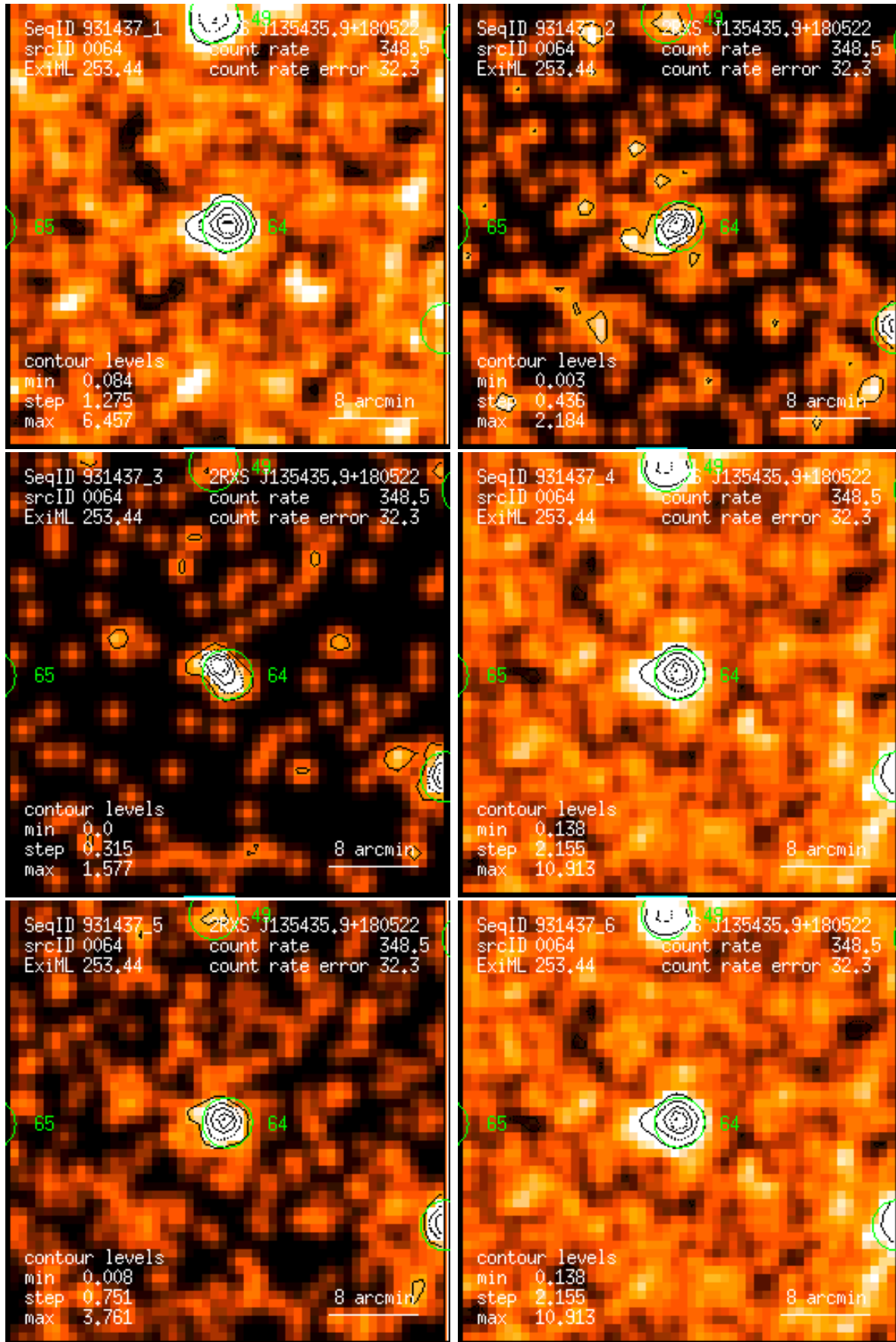
Figure 64: RASS 931437: detection 0064: band rate images, Gaussian filter: (1) PSPC channels 11 – 41, (2) 52 – 90, (3) 91 – 201, (4) 11 – 235, (5) 52 – 201, (6) 11 – 201. Broad band rates in counts/ks. Band rate contour levels in counts/ks/arcmin 2 .
