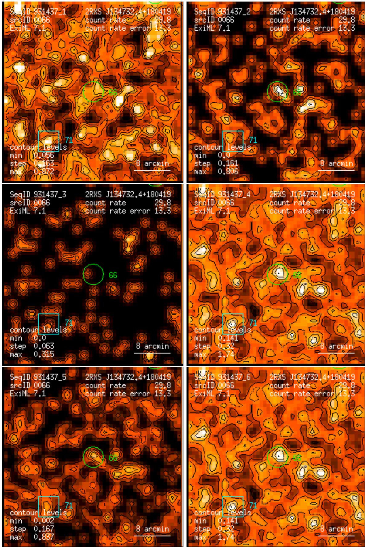
Figure 66: RASS 931437: detection 0066: band rate images, Gaussian filter: (1) PSPC channels 11 – 41, (2) 52 – 90, (3) 91 – 201, (4) 11 – 235, (5) 52 – 201, (6) 11 – 201. Broad band rates in counts/ks. Band rate contour levels in counts/ks/arcmin 2 .
