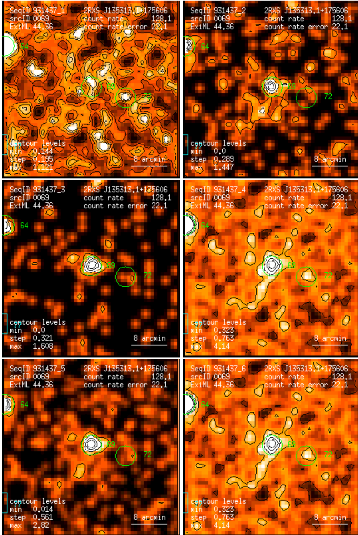
Figure 69: RASS 931437: detection 0069: band rate images, Gaussian filter: (1) PSPC channels 11 – 41, (2) 52 – 90, (3) 91 – 201, (4) 11 – 235, (5) 52 – 201, (6) 11 – 201. Broad band rates in counts/ks. Band rate contour levels in counts/ks/arcmin 2 .
