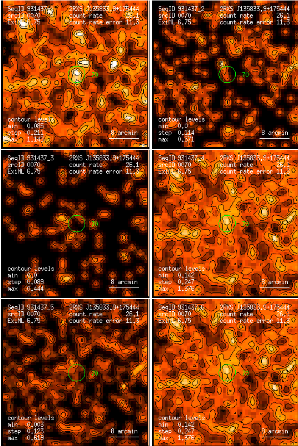
Figure 70: RASS 931437: detection 0070: band rate images, Gaussian filter: (1) PSPC channels 11 – 41, (2) 52 – 90, (3) 91 – 201, (4) 11 – 235, (5) 52 – 201, (6) 11 – 201. Broad band rates in counts/ks. Band rate contour levels in counts/ks/arcmin 2 .
