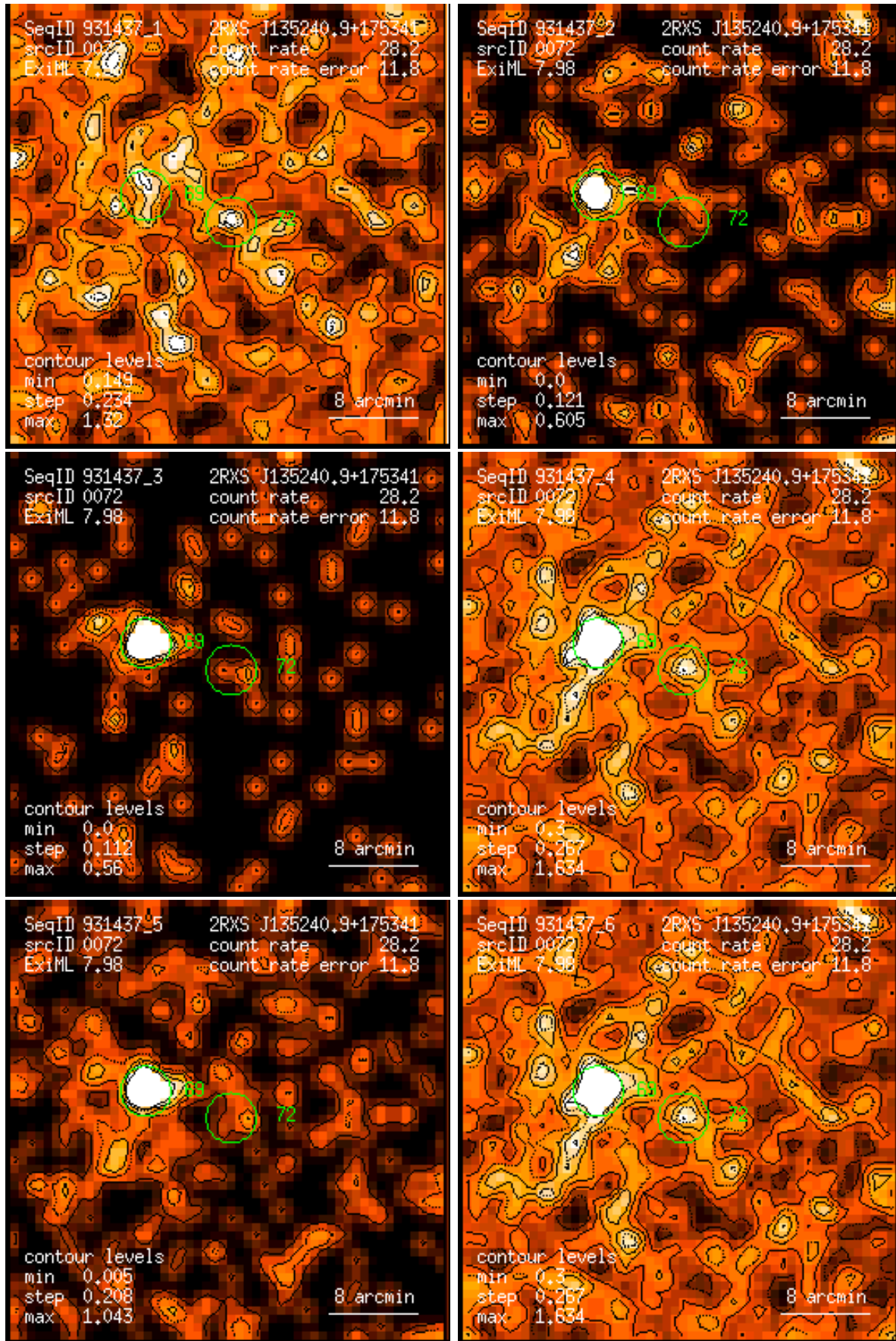
Figure 72: RASS 931437: detection 0072: band rate images, Gaussian filter: (1) PSPC channels 11 – 41, (2) 52 – 90, (3) 91 – 201, (4) 11 – 235, (5) 52 – 201, (6) 11 – 201. Broad band rates in counts/ks. Band rate contour levels in counts/ks/arcmin 2 .
