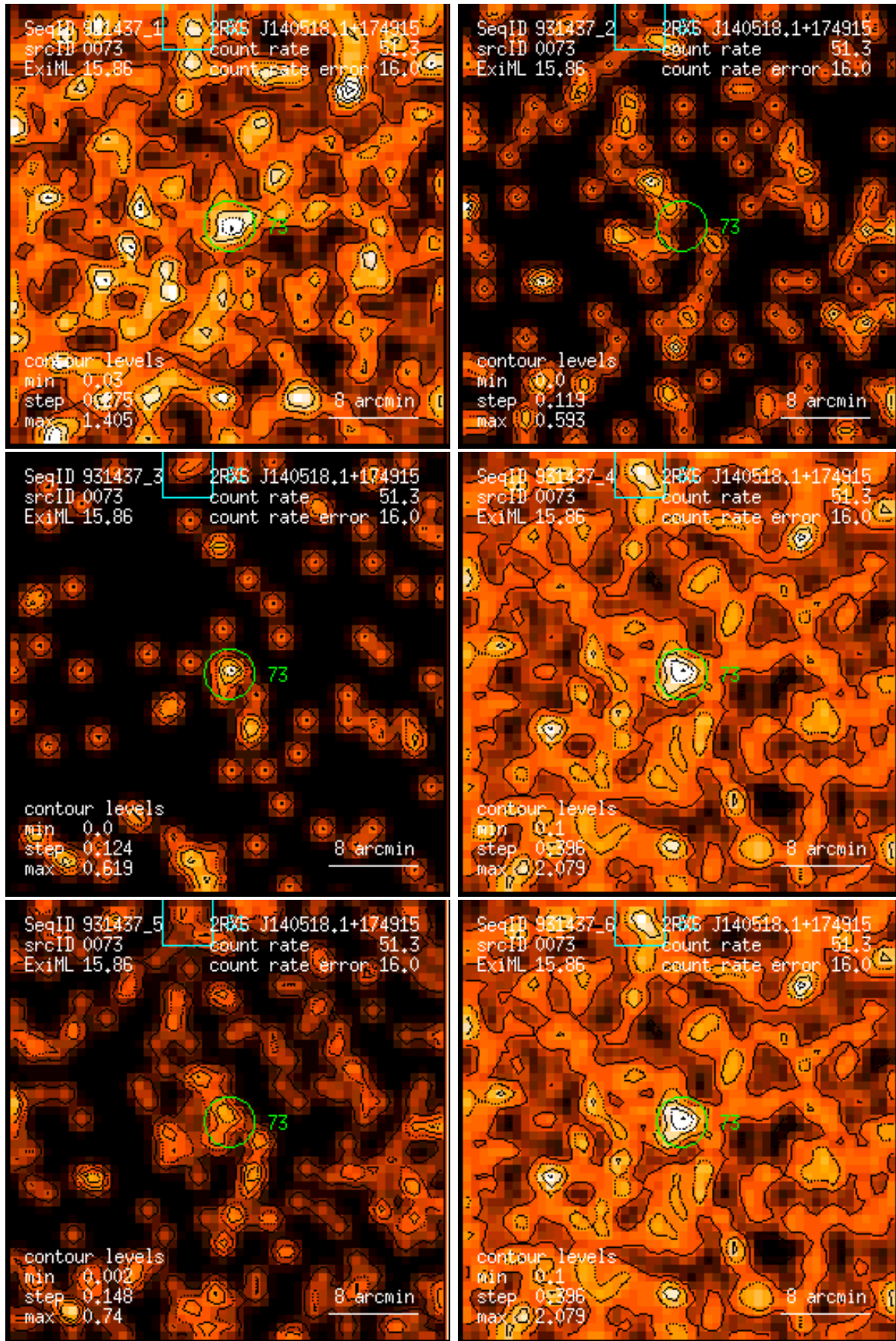
Figure 73: RASS 931437: detection 0073: band rate images, Gaussian filter: (1) PSPC channels 11 – 41, (2) 52 – 90, (3) 91 – 201, (4) 11 – 235, (5) 52 – 201, (6) 11 – 201. Broad band rates in counts/ks. Band rate contour levels in counts/ks/arcmin 2 .
