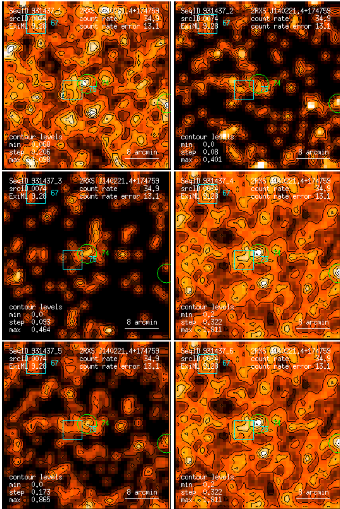
Figure 74: RASS 931437: detection 0074: band rate images, Gaussian filter: (1) PSPC channels 11 – 41, (2) 52 – 90, (3) 91 – 201, (4) 11 – 235, (5) 52 – 201, (6) 11 – 201. Broad band rates in counts/ks. Band rate contour levels in counts/ks/arcmin 2 .
