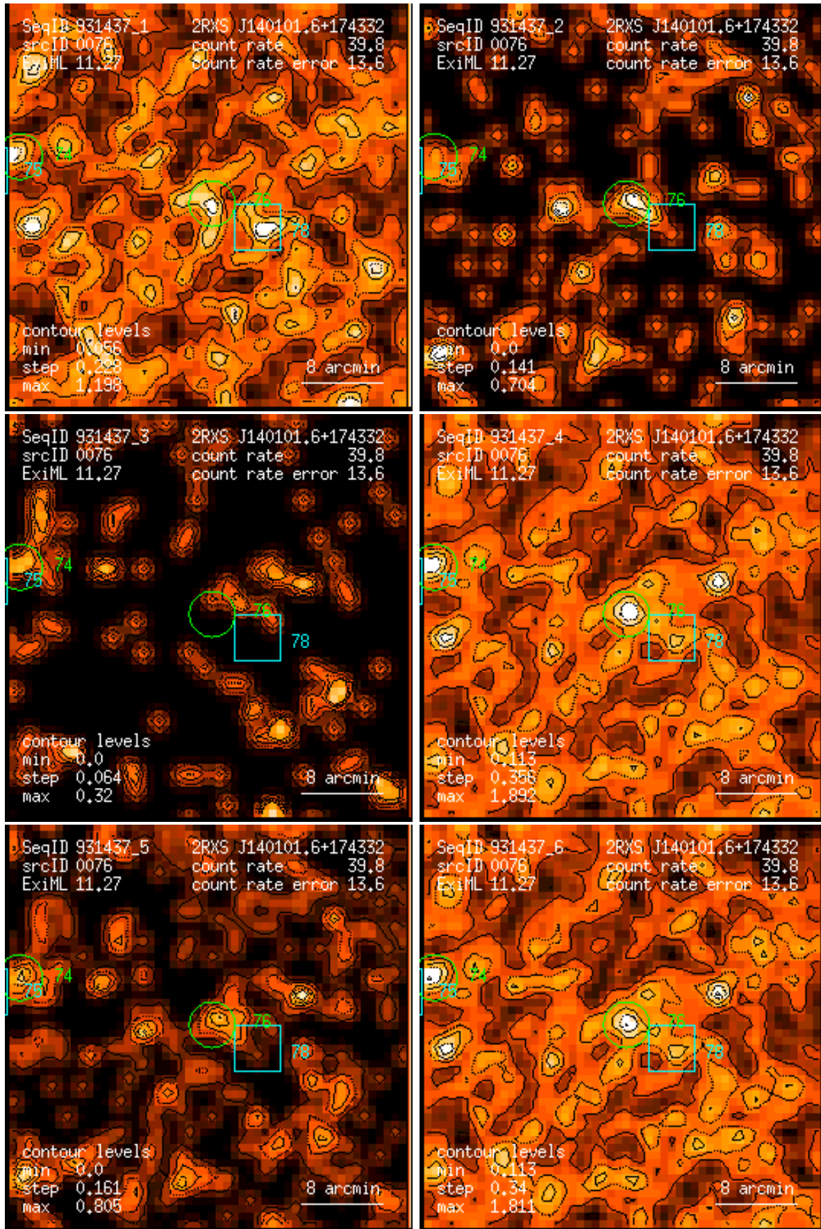
Figure 76: RASS 931437: detection 0076: band rate images, Gaussian filter: (1) PSPC channels 11 – 41, (2) 52 – 90, (3) 91 – 201, (4) 11 – 235, (5) 52 – 201, (6) 11 – 201. Broad band rates in counts/ks. Band rate contour levels in counts/ks/arcmin 2 .
