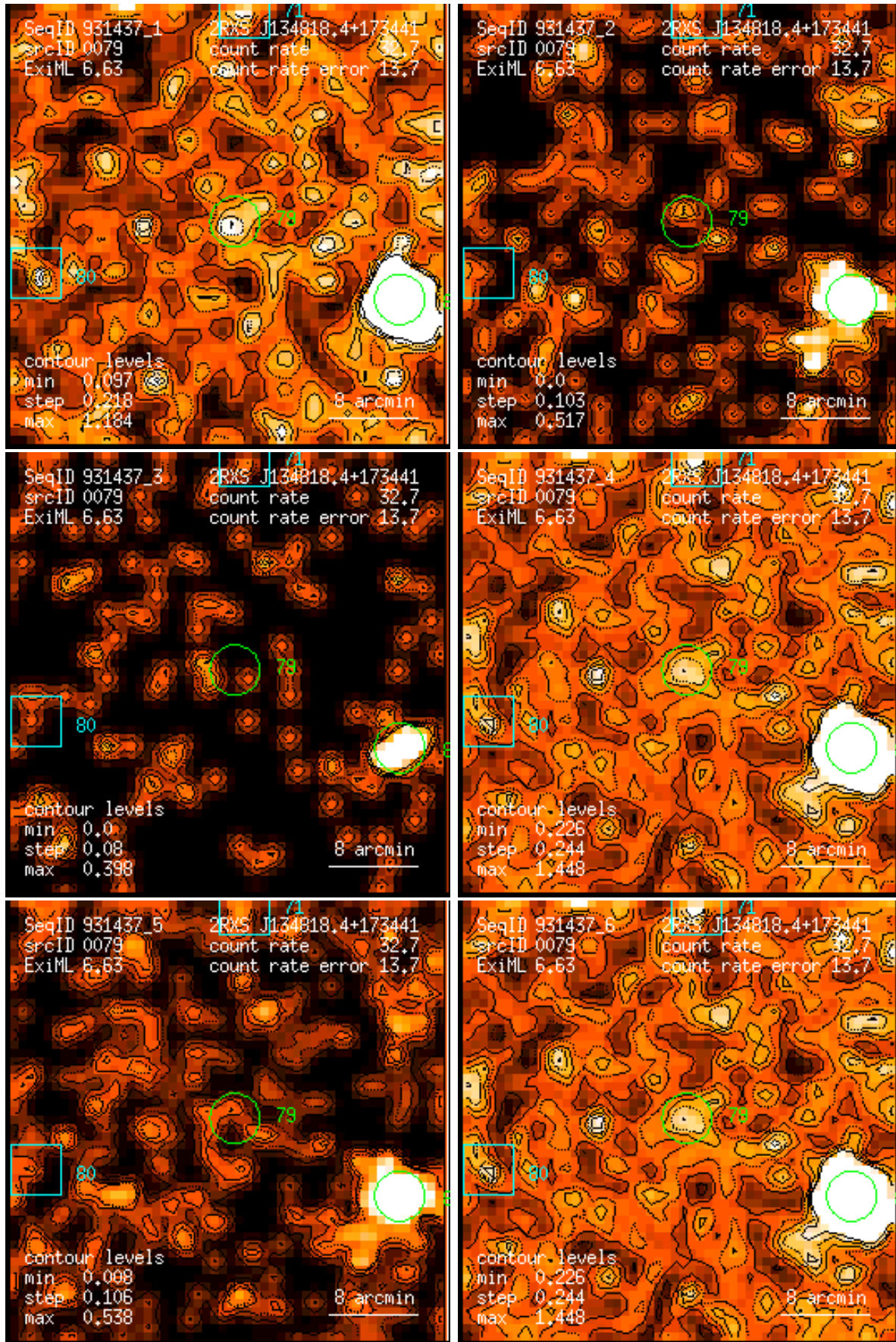
Figure 79: RASS 931437: detection 0079: band rate images, Gaussian filter: (1) PSPC channels 11 – 41, (2) 52 – 90, (3) 91 – 201, (4) 11 – 235, (5) 52 – 201, (6) 11 – 201. Broad band rates in counts/ks. Band rate contour levels in counts/ks/arcmin 2 .
