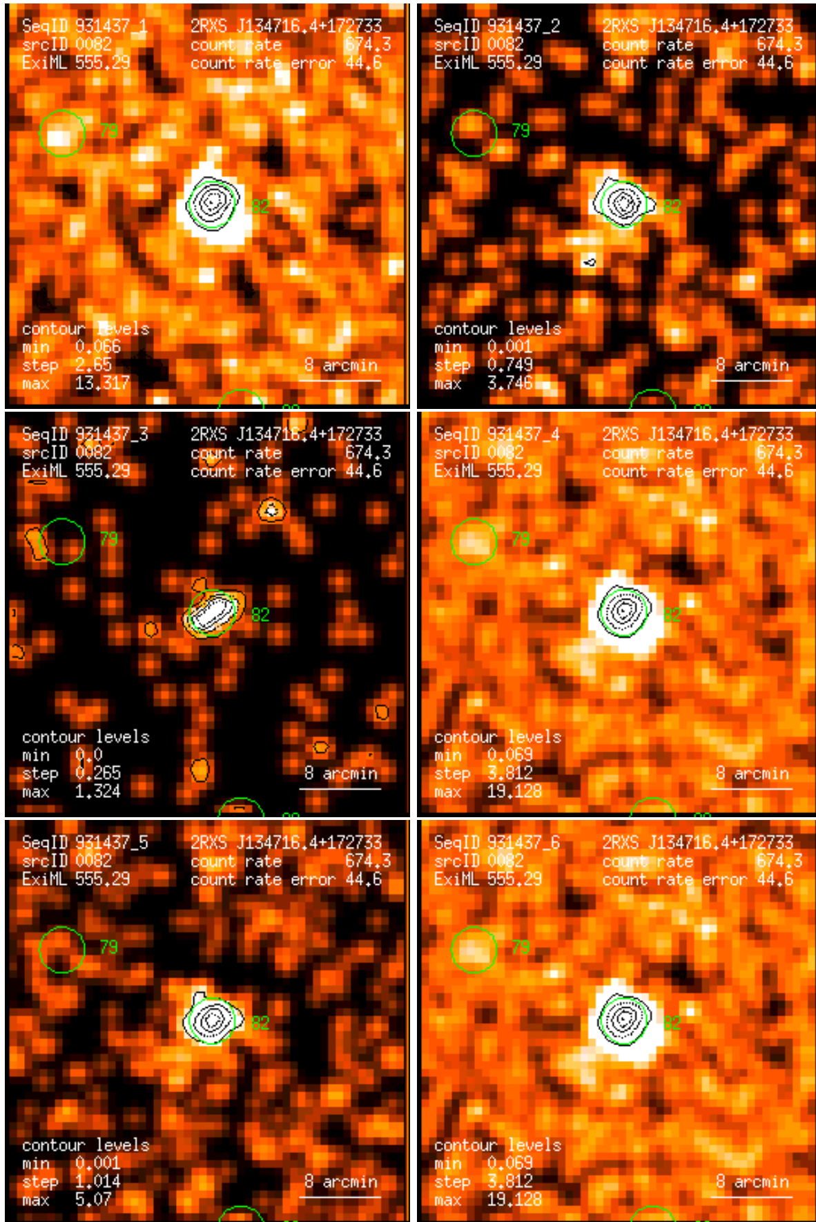
Figure 82: RASS 931437: detection 0082: band rate images, Gaussian filter: (1) PSPC channels 11 – 41, (2) 52 – 90, (3) 91 – 201, (4) 11 – 235, (5) 52 – 201, (6) 11 – 201. Broad band rates in counts/ks. Band rate contour levels in counts/ks/arcmin 2 .
