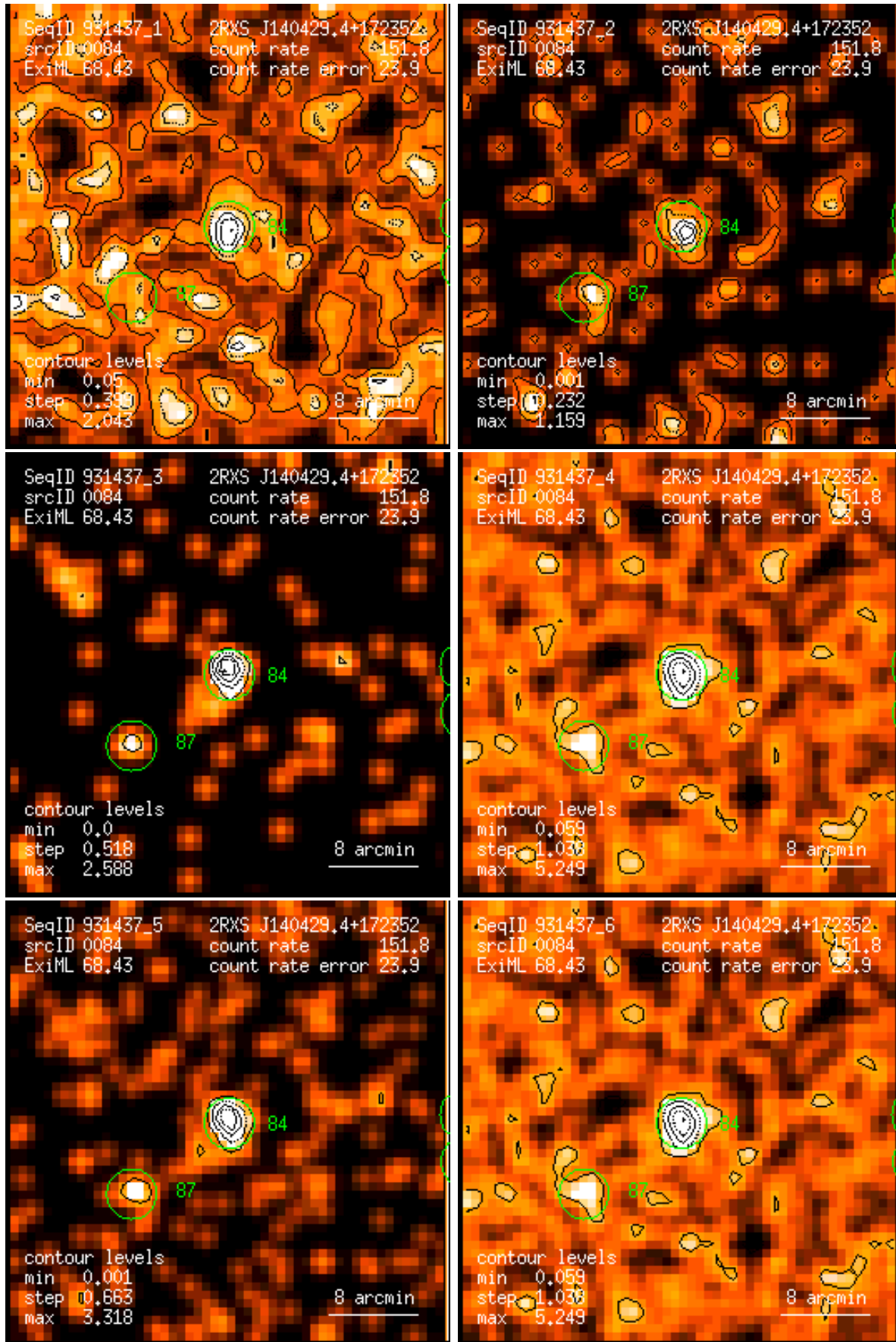
Figure 84: RASS 931437: detection 0084: band rate images, Gaussian filter: (1) PSPC channels 11 – 41, (2) 52 – 90, (3) 91 – 201, (4) 11 – 235, (5) 52 – 201, (6) 11 – 201. Broad band rates in counts/ks. Band rate contour levels in counts/ks/arcmin 2 .
