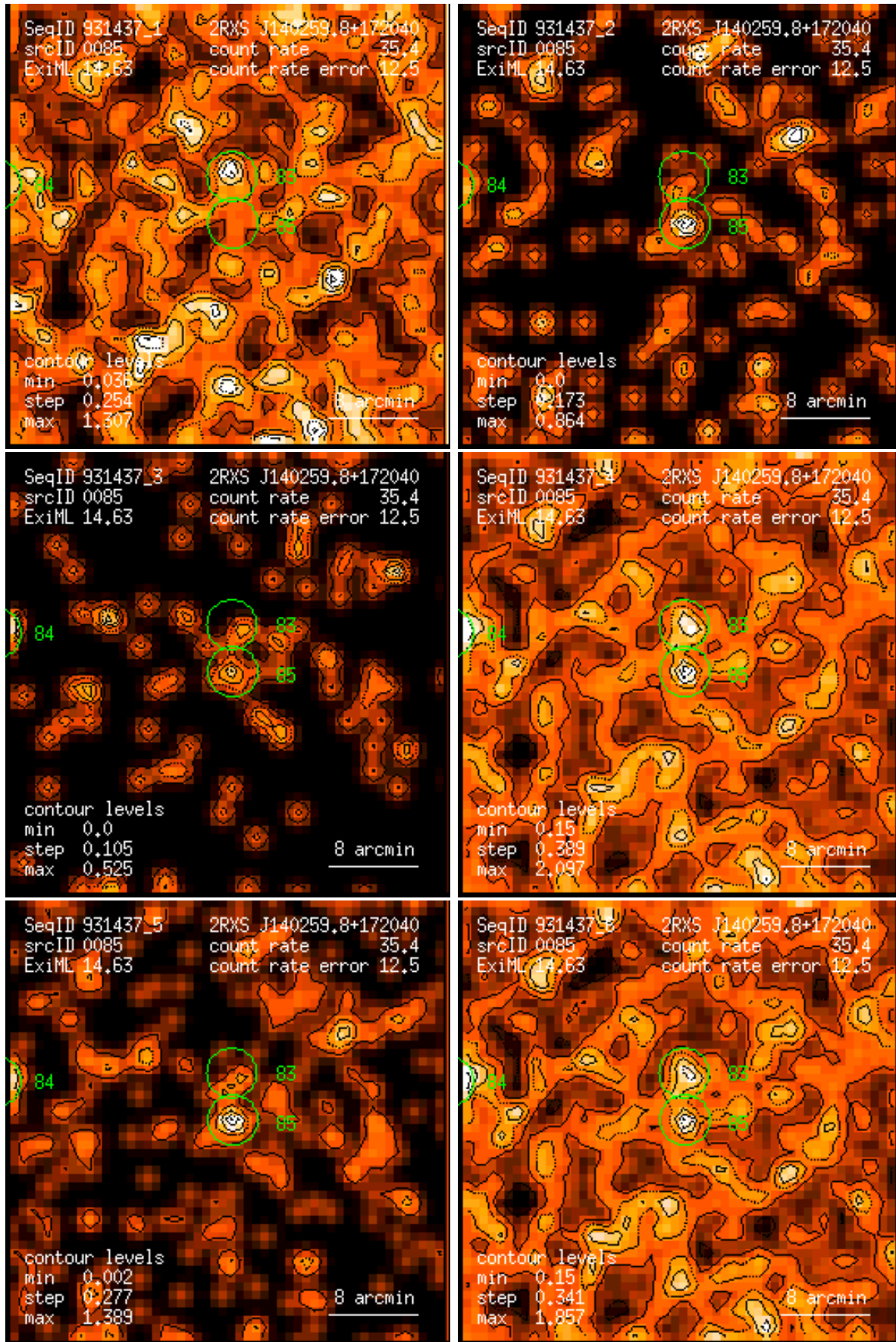
Figure 85: RASS 931437: detection 0085: band rate images, Gaussian filter: (1) PSPC channels 11 – 41, (2) 52 – 90, (3) 91 – 201, (4) 11 – 235, (5) 52 – 201, (6) 11 – 201. Broad band rates in counts/ks. Band rate contour levels in counts/ks/arcmin 2 .
