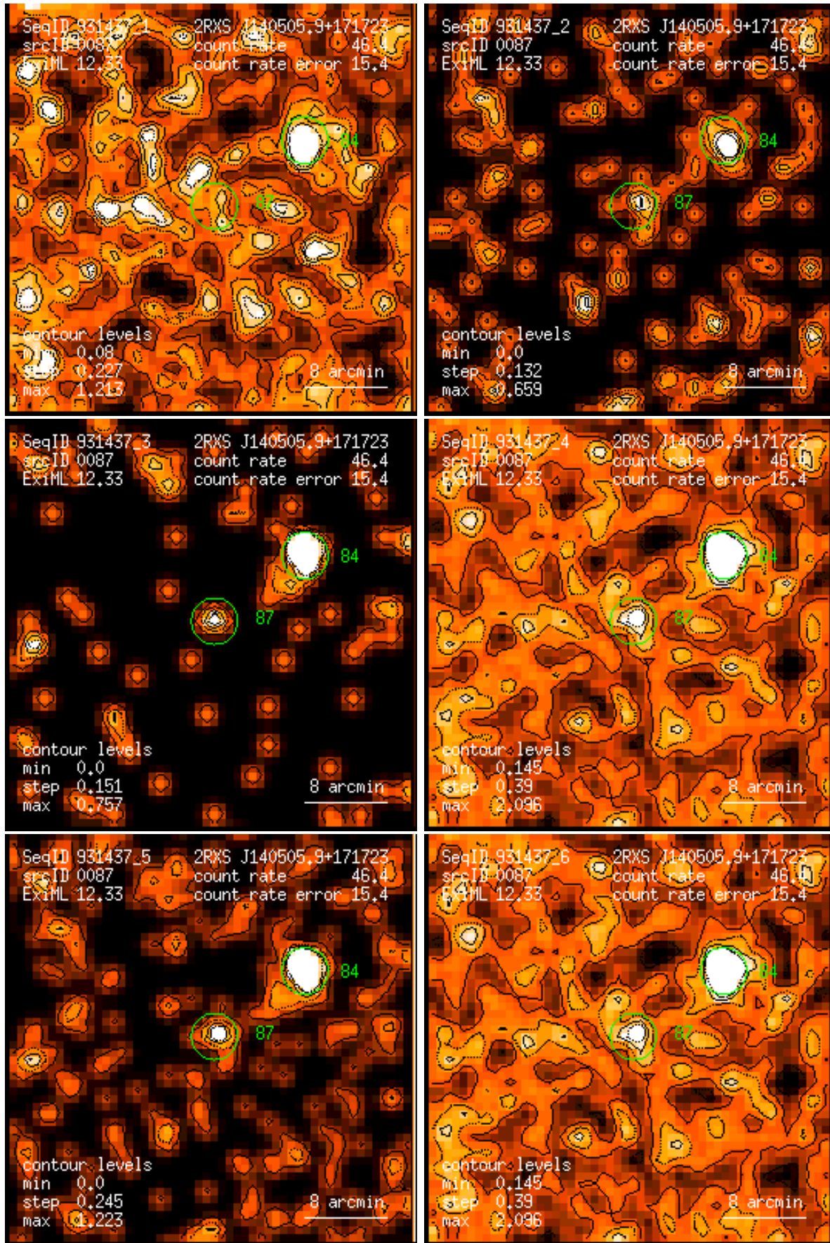
Figure 87: RASS 931437: detection 0087: band rate images, Gaussian filter: (1) PSPC channels 11 – 41, (2) 52 – 90, (3) 91 – 201, (4) 11 – 235, (5) 52 – 201, (6) 11 – 201. Broad band rates in counts/ks. Band rate contour levels in counts/ks/arcmin 2 .
