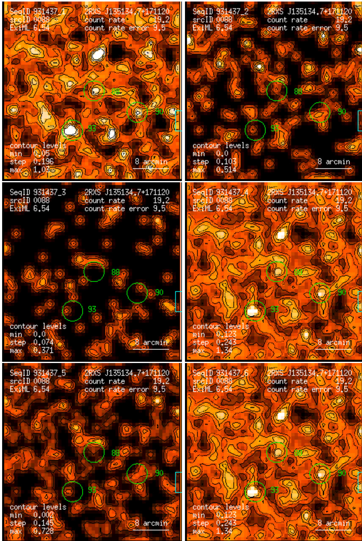
Figure 88: RASS 931437: detection 0088: band rate images, Gaussian filter: (1) PSPC channels 11 – 41, (2) 52 – 90, (3) 91 – 201, (4) 11 – 235, (5) 52 – 201, (6) 11 – 201. Broad band rates in counts/ks. Band rate contour levels in counts/ks/arcmin 2 .
