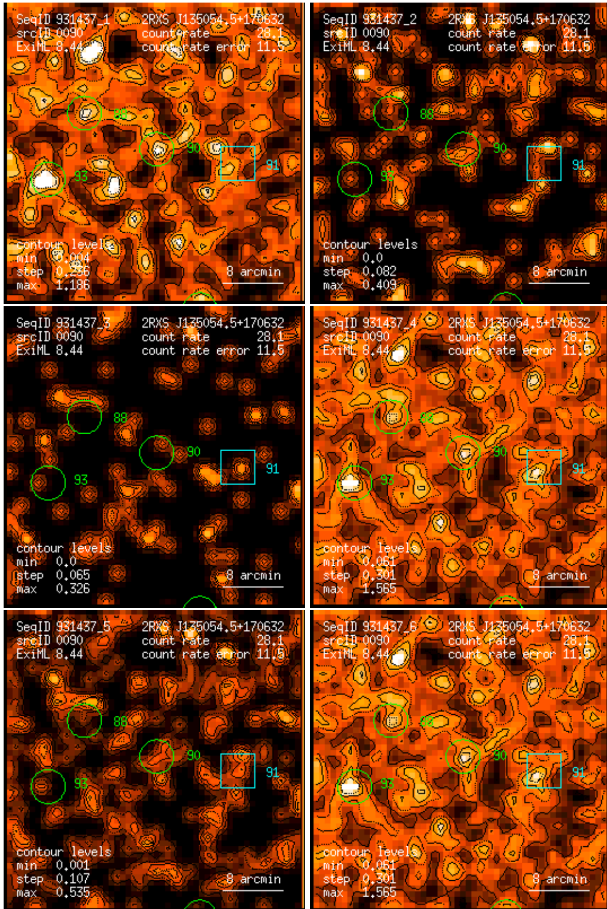
Figure 90: RASS 931437: detection 0090: band rate images, Gaussian filter: (1) PSPC channels 11 – 41, (2) 52 – 90, (3) 91 – 201, (4) 11 – 235, (5) 52 – 201, (6) 11 – 201. Broad band rates in counts/ks. Band rate contour levels in counts/ks/arcmin 2 .
