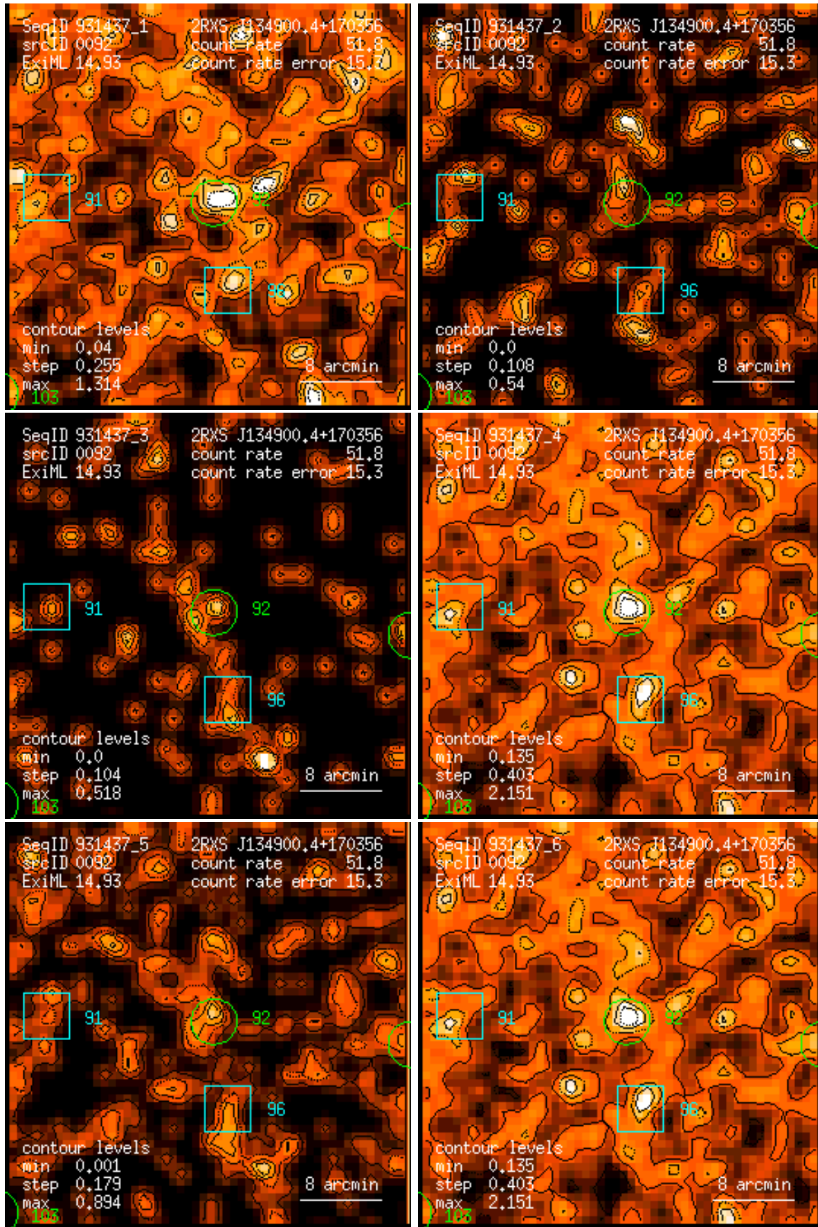
Figure 92: RASS 931437: detection 0092: band rate images, Gaussian filter: (1) PSPC channels 11 – 41, (2) 52 – 90, (3) 91 – 201, (4) 11 – 235, (5) 52 – 201, (6) 11 – 201. Broad band rates in counts/ks. Band rate contour levels in counts/ks/arcmin 2 .
