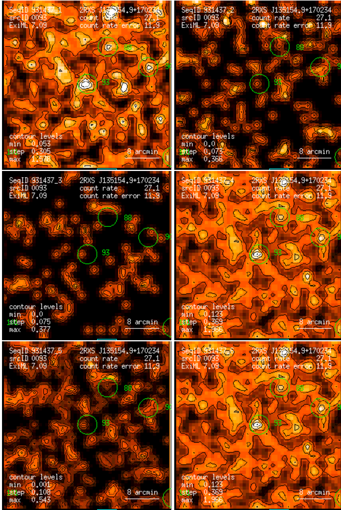
Figure 93: RASS 931437: detection 0093: band rate images, Gaussian filter: (1) PSPC channels 11 – 41, (2) 52 – 90, (3) 91 – 201, (4) 11 – 235, (5) 52 – 201, (6) 11 – 201. Broad band rates in counts/ks. Band rate contour levels in counts/ks/arcmin 2 .
