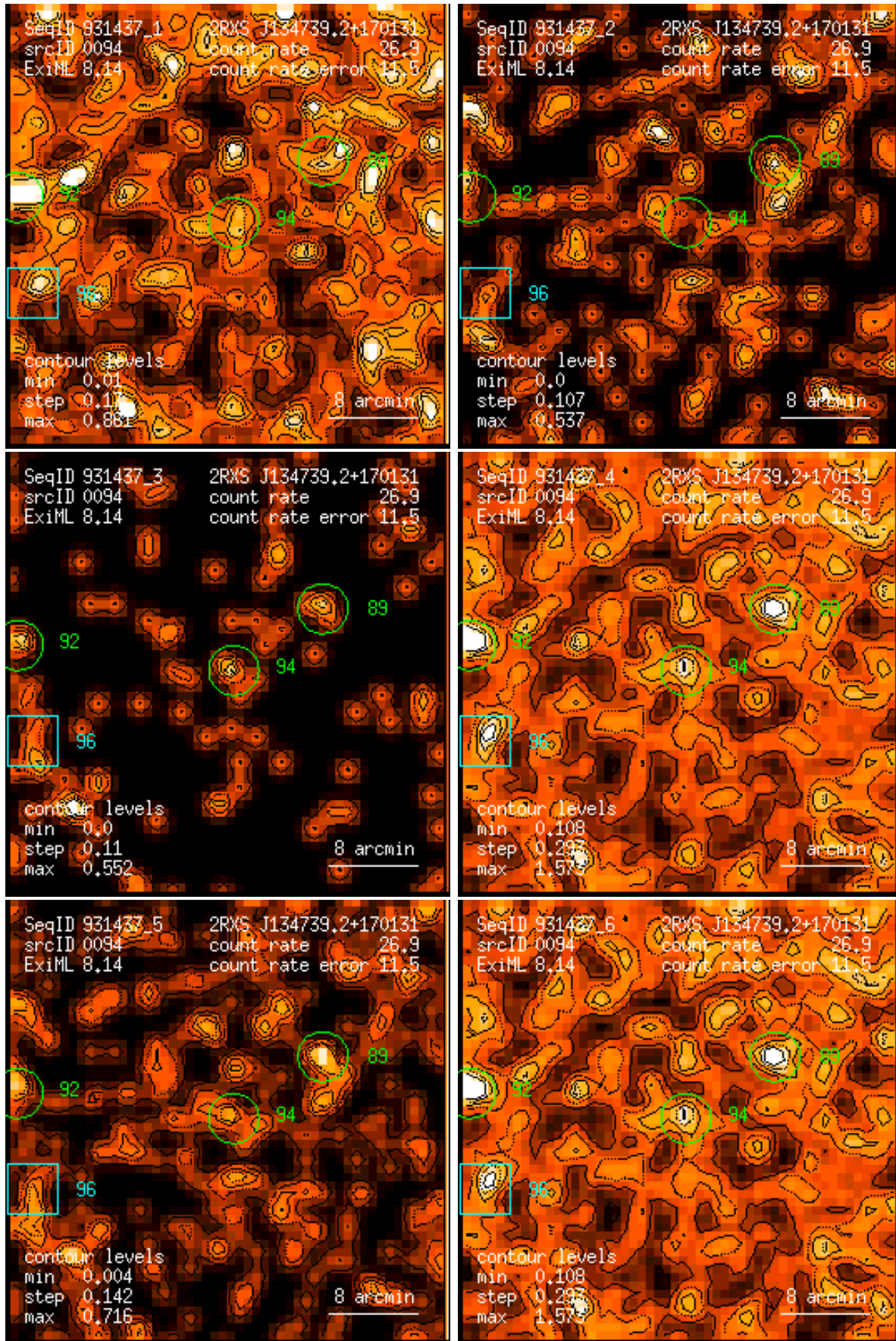
Figure 94: RASS 931437: detection 0094: band rate images, Gaussian filter: (1) PSPC channels 11 – 41, (2) 52 – 90, (3) 91 – 201, (4) 11 – 235, (5) 52 – 201, (6) 11 – 201. Broad band rates in counts/ks. Band rate contour levels in counts/ks/arcmin 2 .
