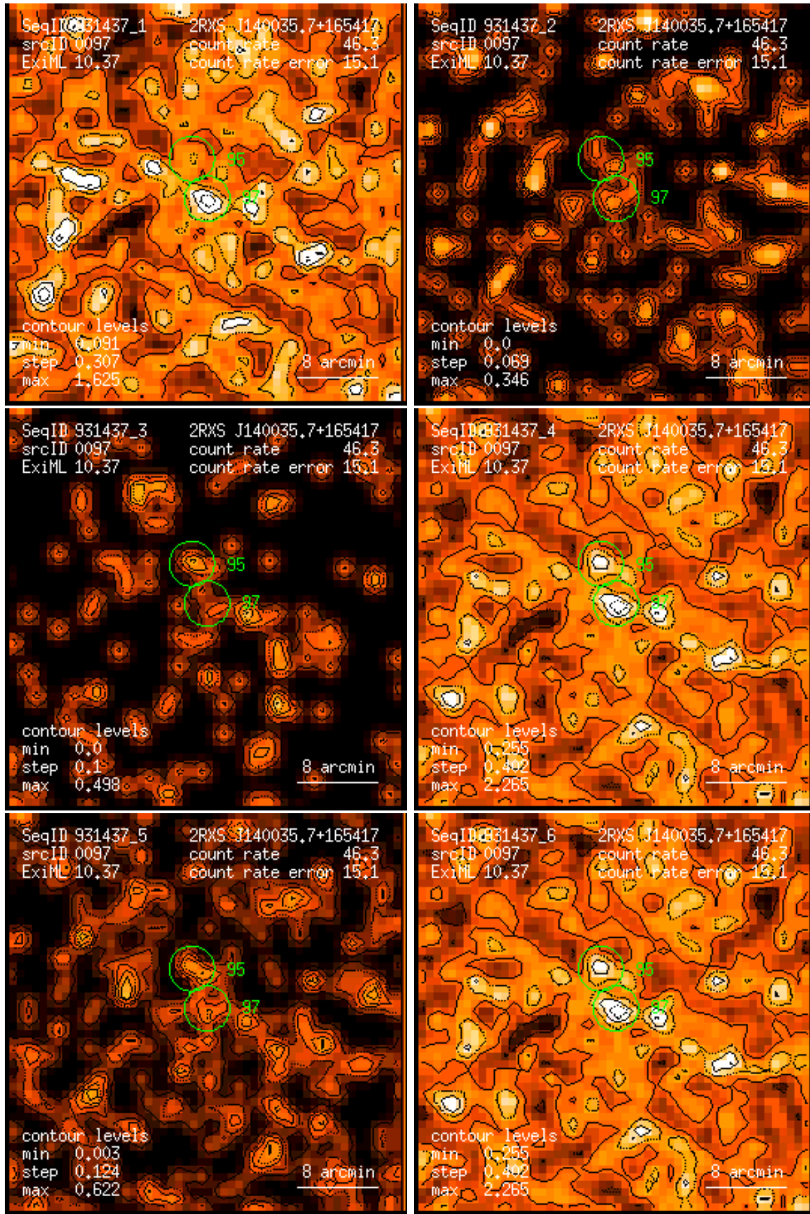
Figure 97: RASS 931437: detection 0097: band rate images, Gaussian filter: (1) PSPC channels 11 – 41, (2) 52 – 90, (3) 91 – 201, (4) 11 – 235, (5) 52 – 201, (6) 11 – 201. Broad band rates in counts/ks. Band rate contour levels in counts/ks/arcmin 2 .
