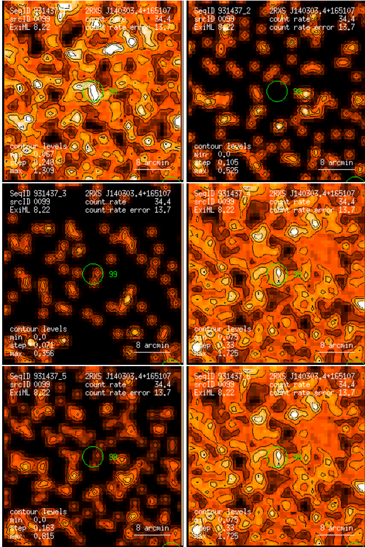
Figure 99: RASS 931437: detection 0099: band rate images, Gaussian filter: (1) PSPC channels 11 – 41, (2) 52 – 90, (3) 91 – 201, (4) 11 – 235, (5) 52 – 201, (6) 11 – 201. Broad band rates in counts/ks. Band rate contour levels in counts/ks/arcmin 2 .
