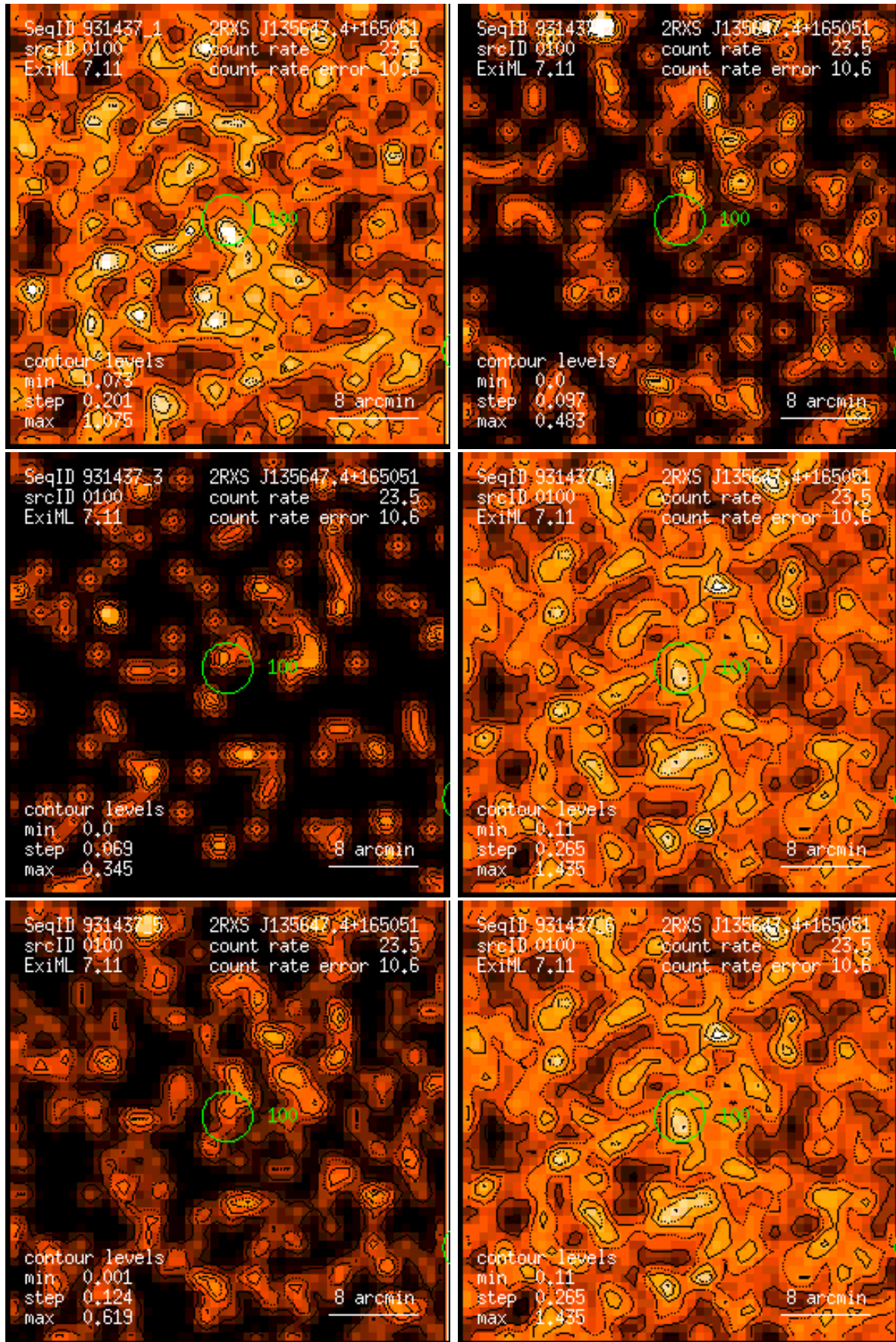
Figure 100: RASS 931437: detection 0100: band rate images, Gaussian filter: (1) PSPC channels 11 – 41, (2) 52 – 90, (3) 91 – 201, (4) 11 – 235, (5) 52 – 201, (6) 11 – 201. Broad band rates in counts/ks. Band rate contour levels in counts/ks/arcmin 2 .
