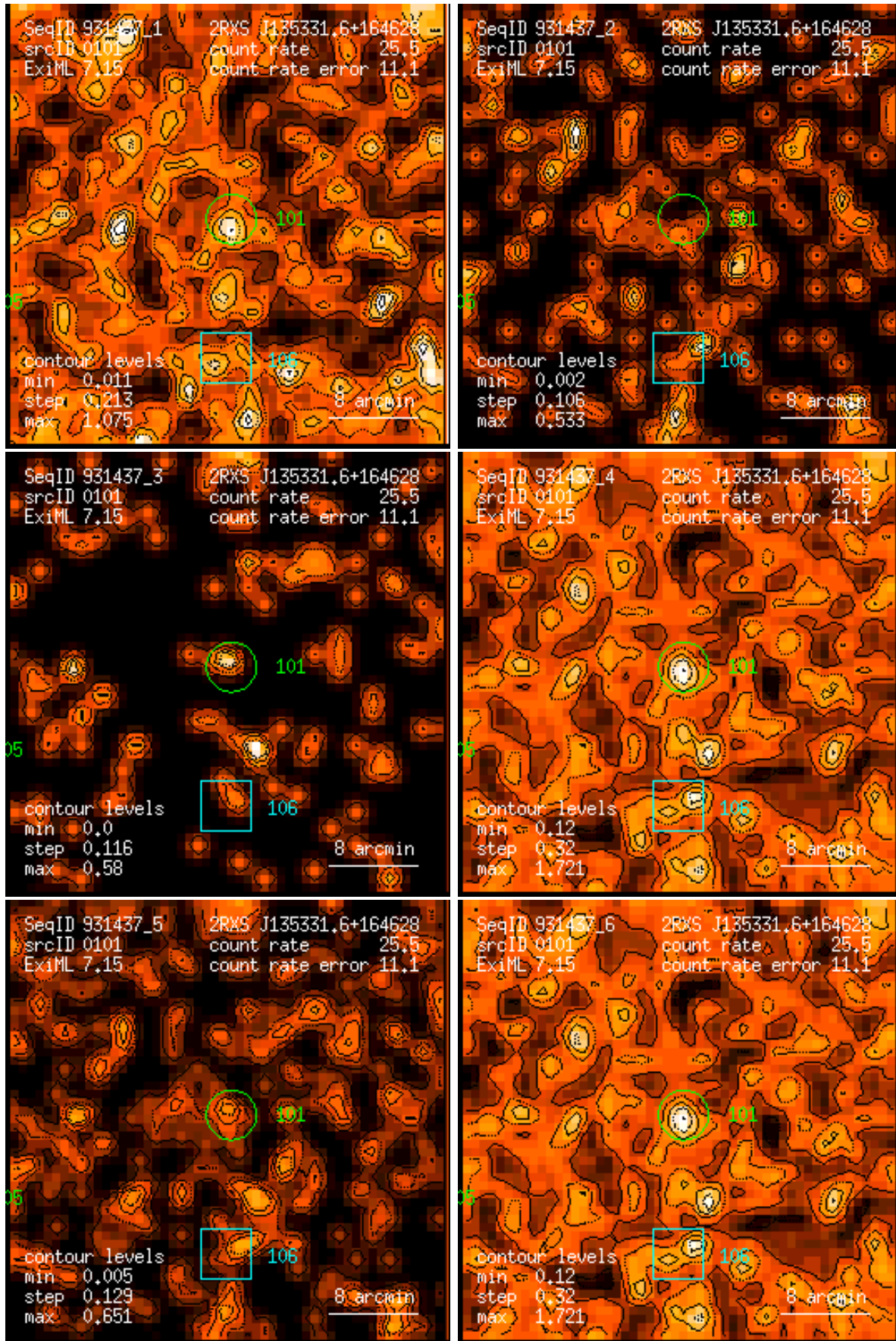
Figure 101: RASS 931437: detection 0101: band rate images, Gaussian filter: (1) PSPC channels 11 – 41, (2) 52 – 90, (3) 91 – 201, (4) 11 – 235, (5) 52 – 201, (6) 11 – 201. Broad band rates in counts/ks. Band rate contour levels in counts/ks/arcmin 2 .
