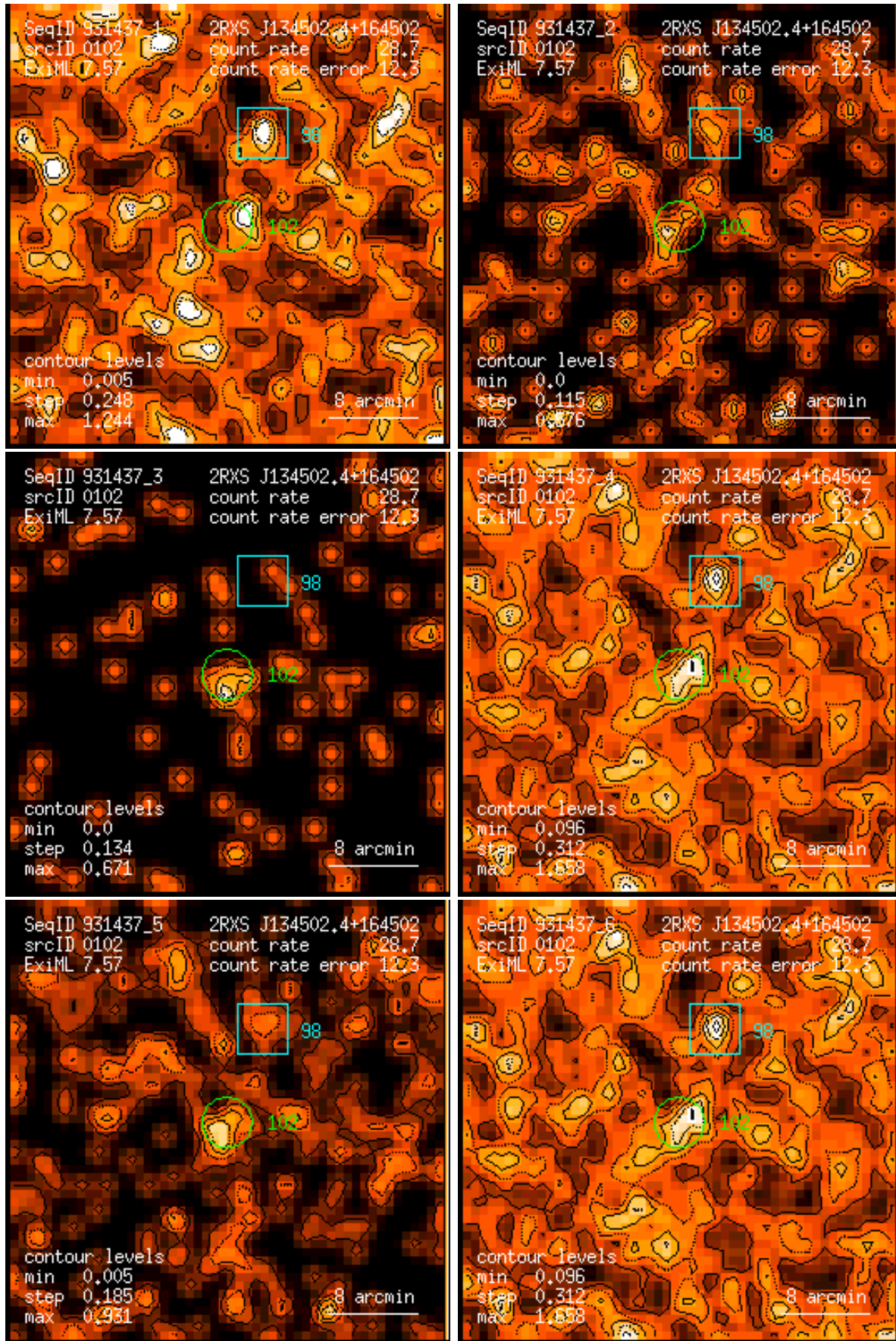
Figure 102: RASS 931437: detection 0102: band rate images, Gaussian filter: (1) PSPC channels 11 – 41, (2) 52 – 90, (3) 91 – 201, (4) 11 – 235, (5) 52 – 201, (6) 11 – 201. Broad band rates in counts/ks. Band rate contour levels in counts/ks/arcmin 2 .
