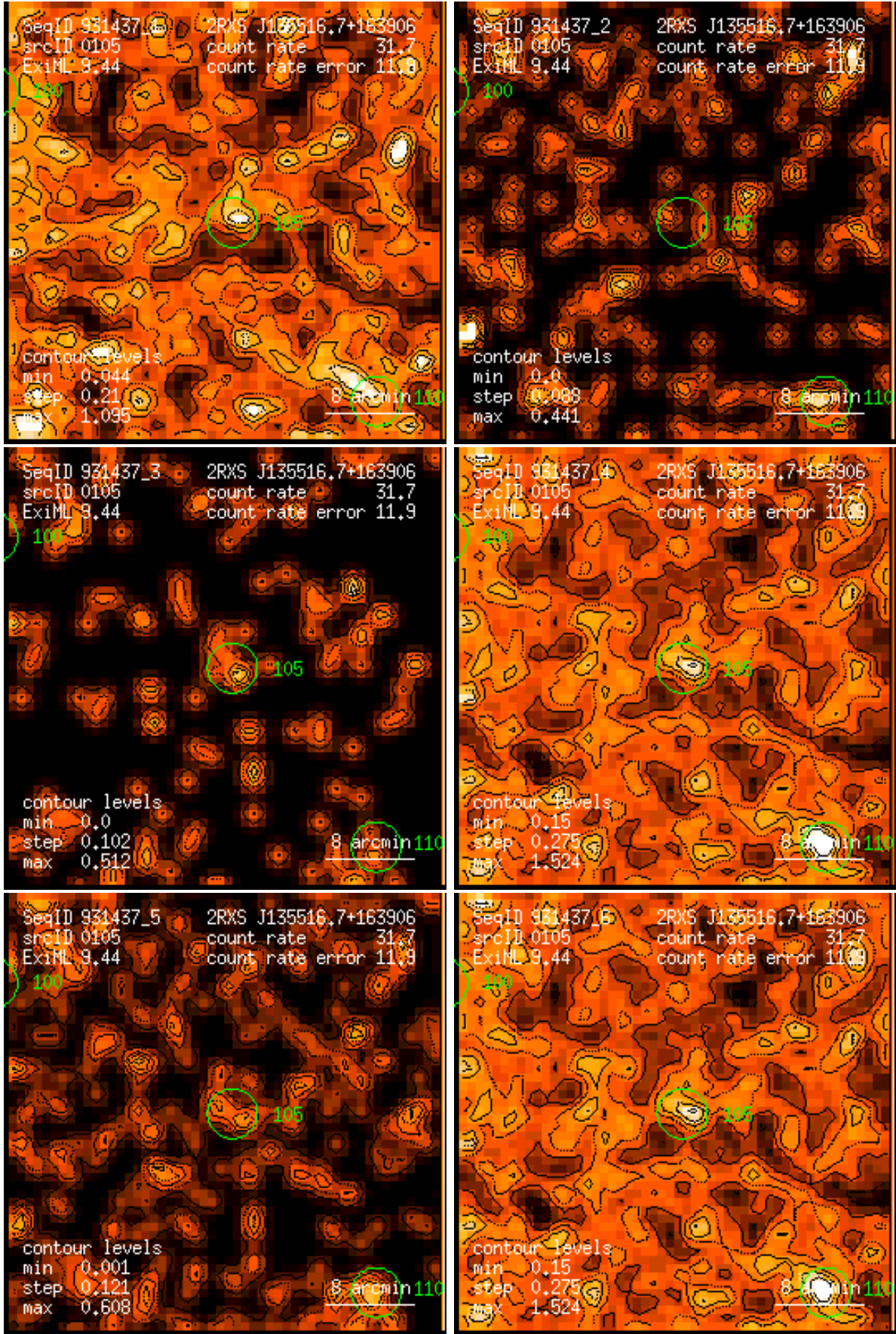
Figure 105: RASS 931437: detection 0105: band rate images, Gaussian filter: (1) PSPC channels 11 – 41, (2) 52 – 90, (3) 91 – 201, (4) 11 – 235, (5) 52 – 201, (6) 11 – 201. Broad band rates in counts/ks. Band rate contour levels in counts/ks/arcmin 2 .
