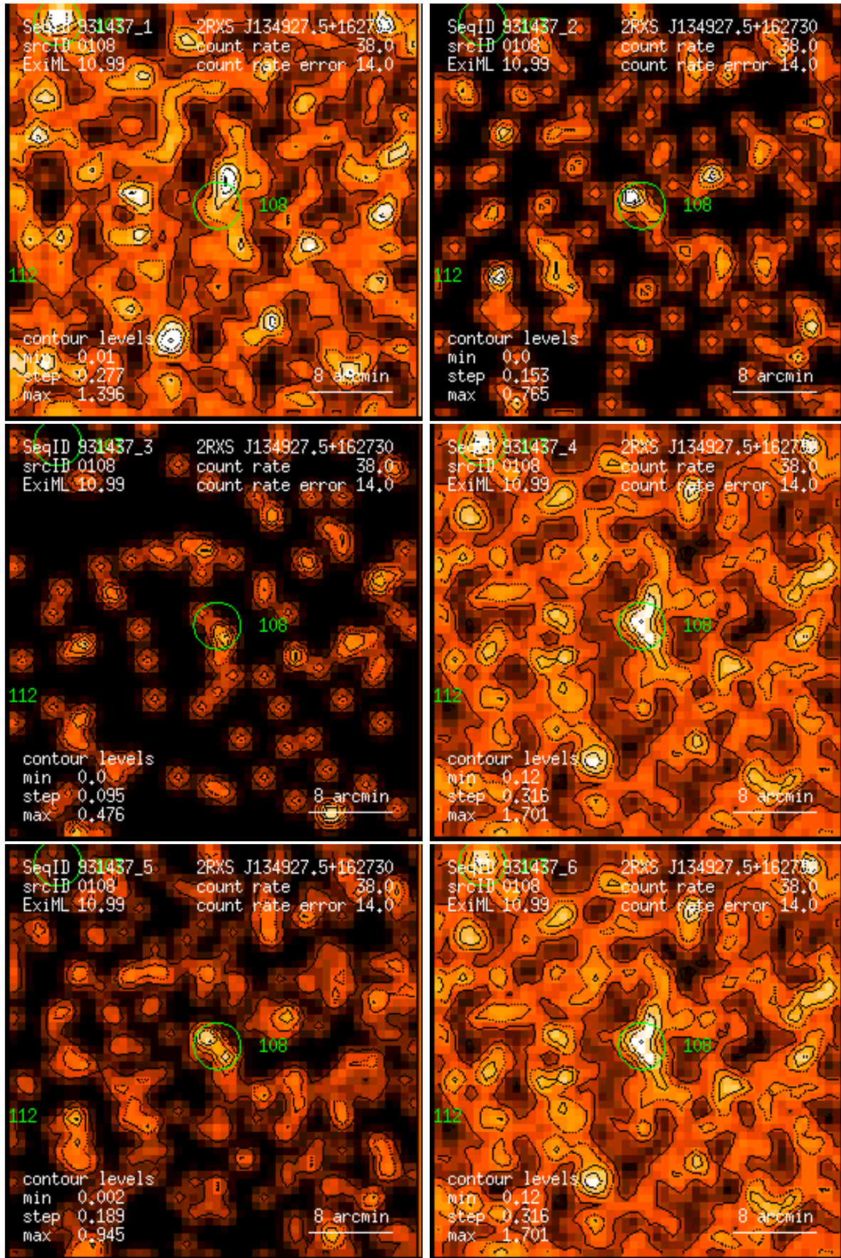
Figure 108: RASS 931437: detection 0108: band rate images, Gaussian filter: (1) PSPC channels 11 – 41, (2) 52 – 90, (3) 91 – 201, (4) 11 – 235, (5) 52 – 201, (6) 11 – 201. Broad band rates in counts/ks. Band rate contour levels in counts/ks/arcmin 2 .
