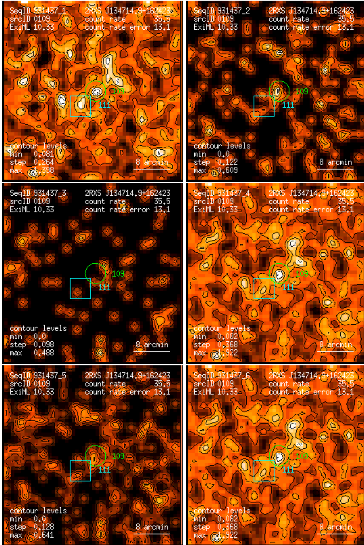
Figure 109: RASS 931437: detection 0109: band rate images, Gaussian filter: (1) PSPC channels 11 – 41, (2) 52 – 90, (3) 91 – 201, (4) 11 – 235, (5) 52 – 201, (6) 11 – 201. Broad band rates in counts/ks. Band rate contour levels in counts/ks/arcmin 2 .
