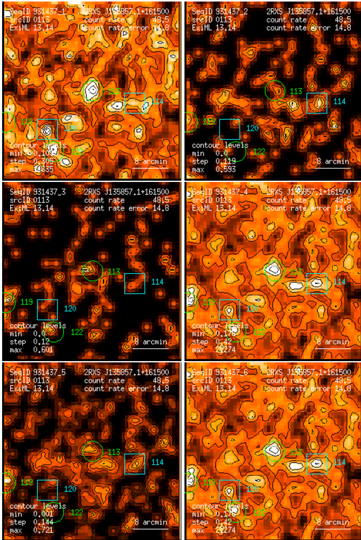
Figure 113: RASS 931437: detection 0113: band rate images, Gaussian filter: (1) PSPC channels 11 – 41, (2) 52 – 90, (3) 91 – 201, (4) 11 – 235, (5) 52 – 201, (6) 11 – 201. Broad band rates in counts/ks. Band rate contour levels in counts/ks/arcmin 2 .
