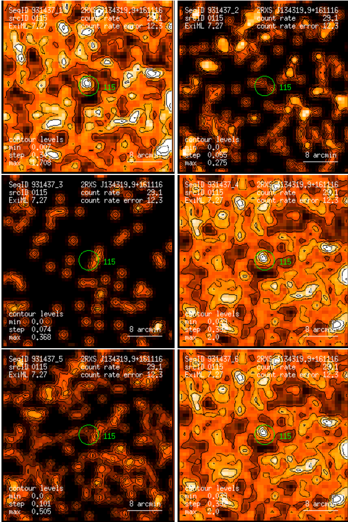
Figure 115: RASS 931437: detection 0115: band rate images, Gaussian filter: (1) PSPC channels 11 – 41, (2) 52 – 90, (3) 91 – 201, (4) 11 – 235, (5) 52 – 201, (6) 11 – 201. Broad band rates in counts/ks. Band rate contour levels in counts/ks/arcmin 2 .
