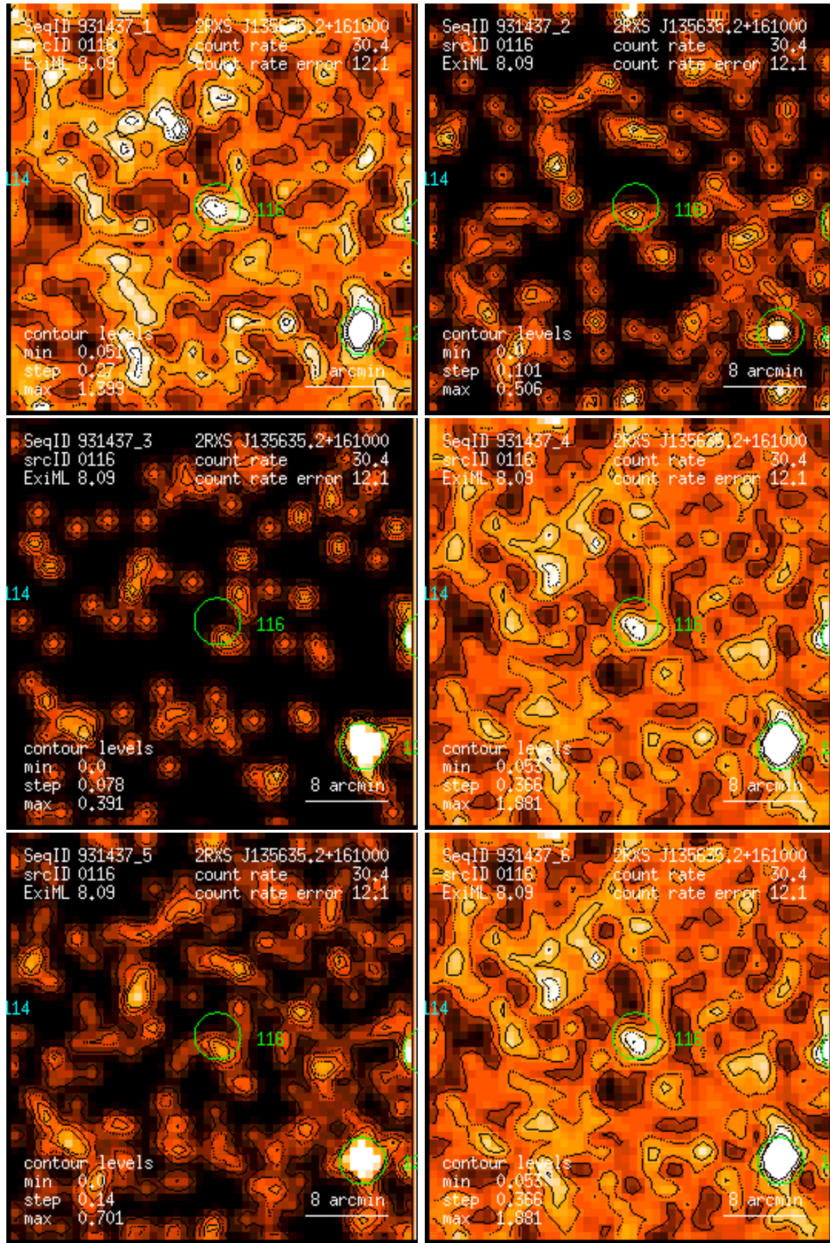
Figure 116: RASS 931437: detection 0116: band rate images, Gaussian filter: (1) PSPC channels 11 – 41, (2) 52 – 90, (3) 91 – 201, (4) 11 – 235, (5) 52 – 201, (6) 11 – 201. Broad band rates in counts/ks. Band rate contour levels in counts/ks/arcmin 2 .
