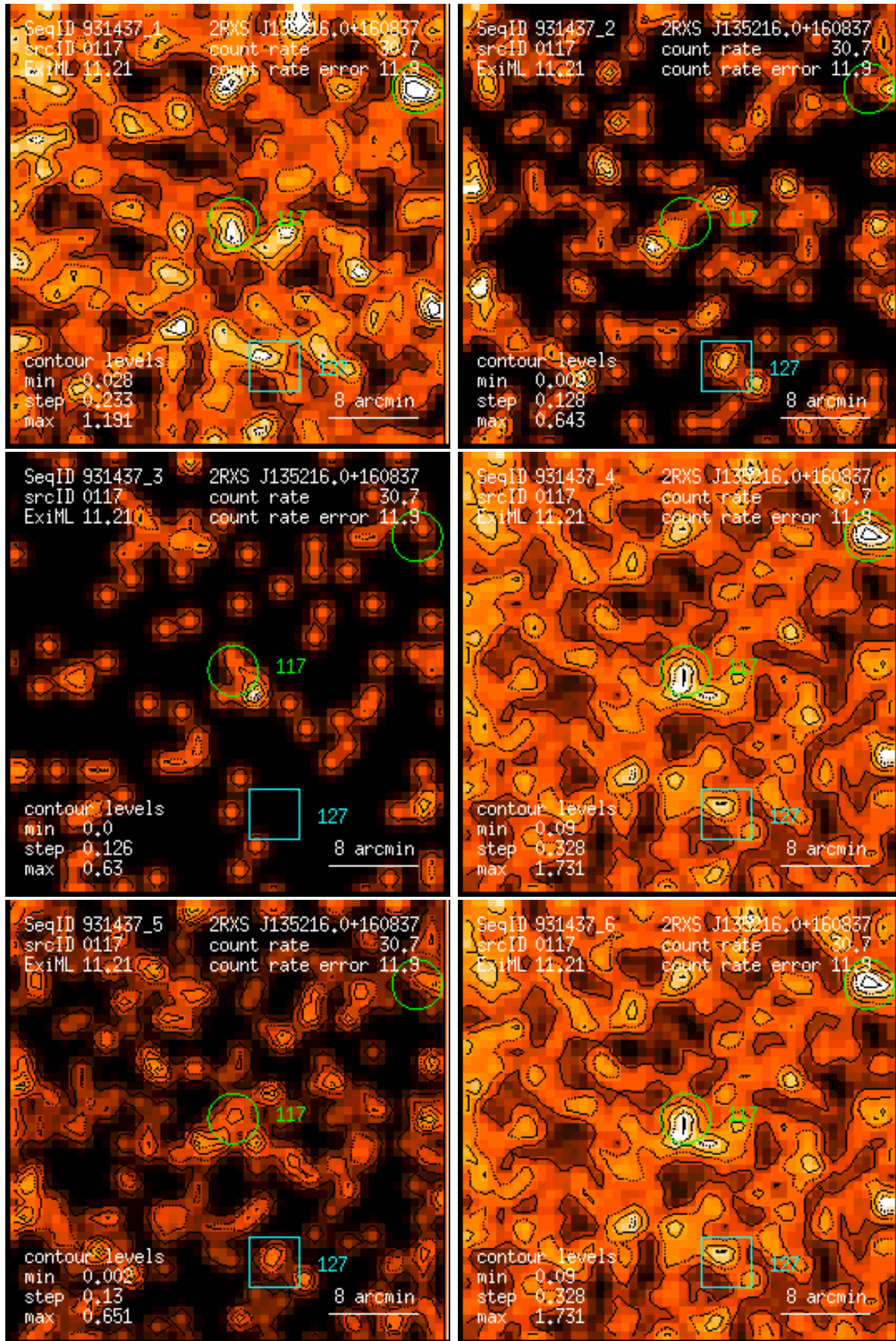
Figure 117: RASS 931437: detection 0117: band rate images, Gaussian filter: (1) PSPC channels 11 – 41, (2) 52 – 90, (3) 91 – 201, (4) 11 – 235, (5) 52 – 201, (6) 11 – 201. Broad band rates in counts/ks. Band rate contour levels in counts/ks/arcmin 2 .
