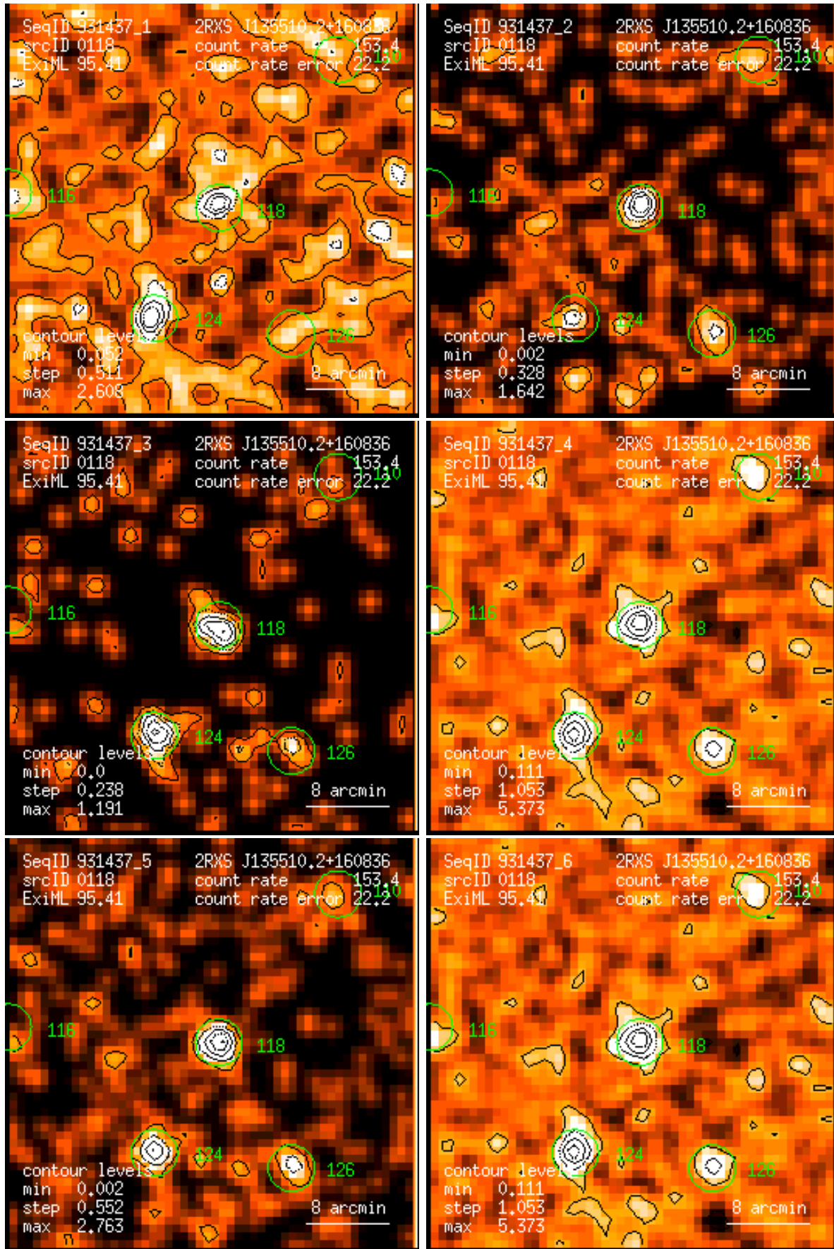
Figure 118: RASS 931437: detection 0118: band rate images, Gaussian filter: (1) PSPC channels 11 – 41, (2) 52 – 90, (3) 91 – 201, (4) 11 – 235, (5) 52 – 201, (6) 11 – 201. Broad band rates in counts/ks. Band rate contour levels in counts/ks/arcmin 2 .
