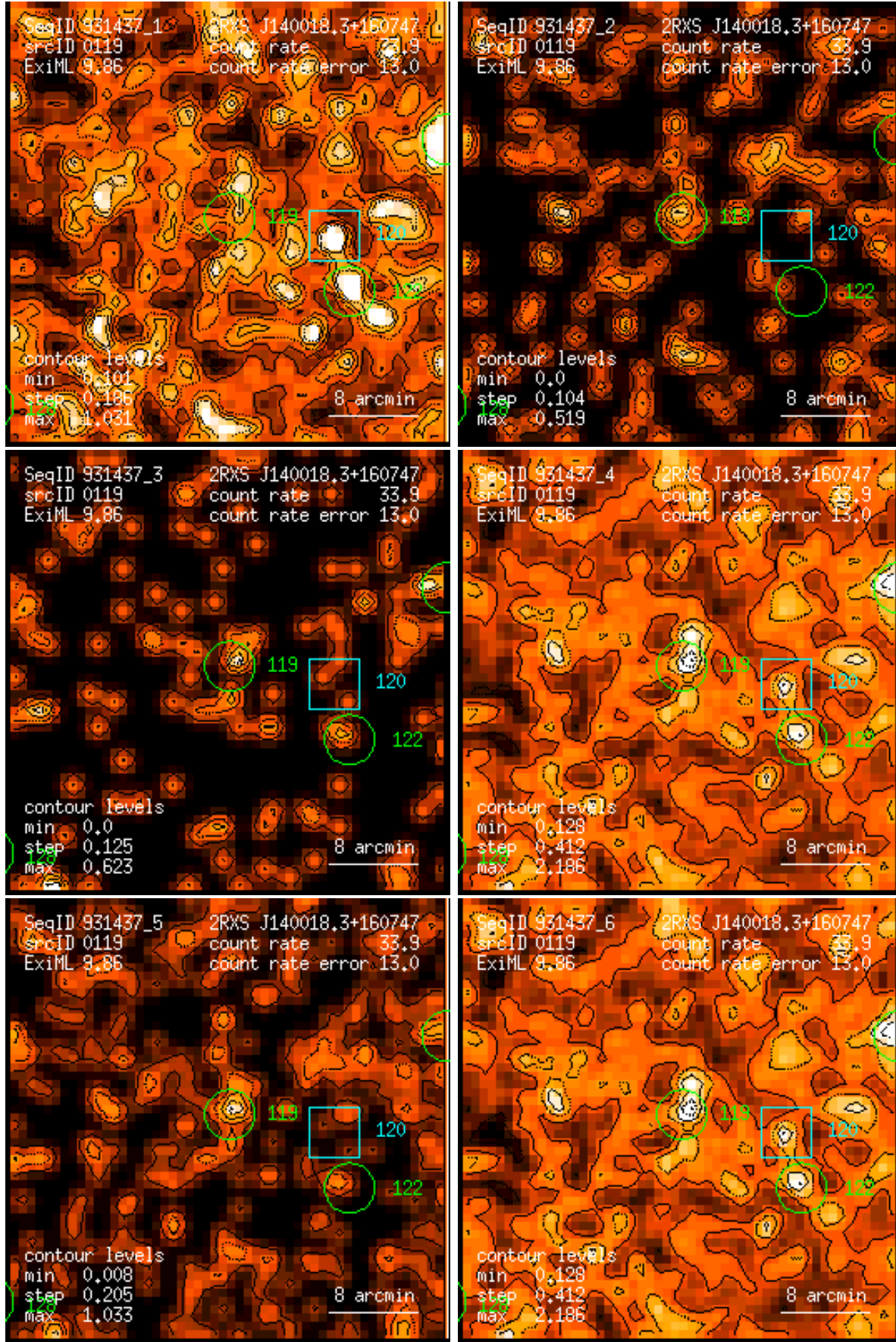
Figure 119: RASS 931437: detection 0119: band rate images, Gaussian filter: (1) PSPC channels 11 – 41, (2) 52 – 90, (3) 91 – 201, (4) 11 – 235, (5) 52 – 201, (6) 11 – 201. Broad band rates in counts/ks. Band rate contour levels in counts/ks/arcmin 2 .
