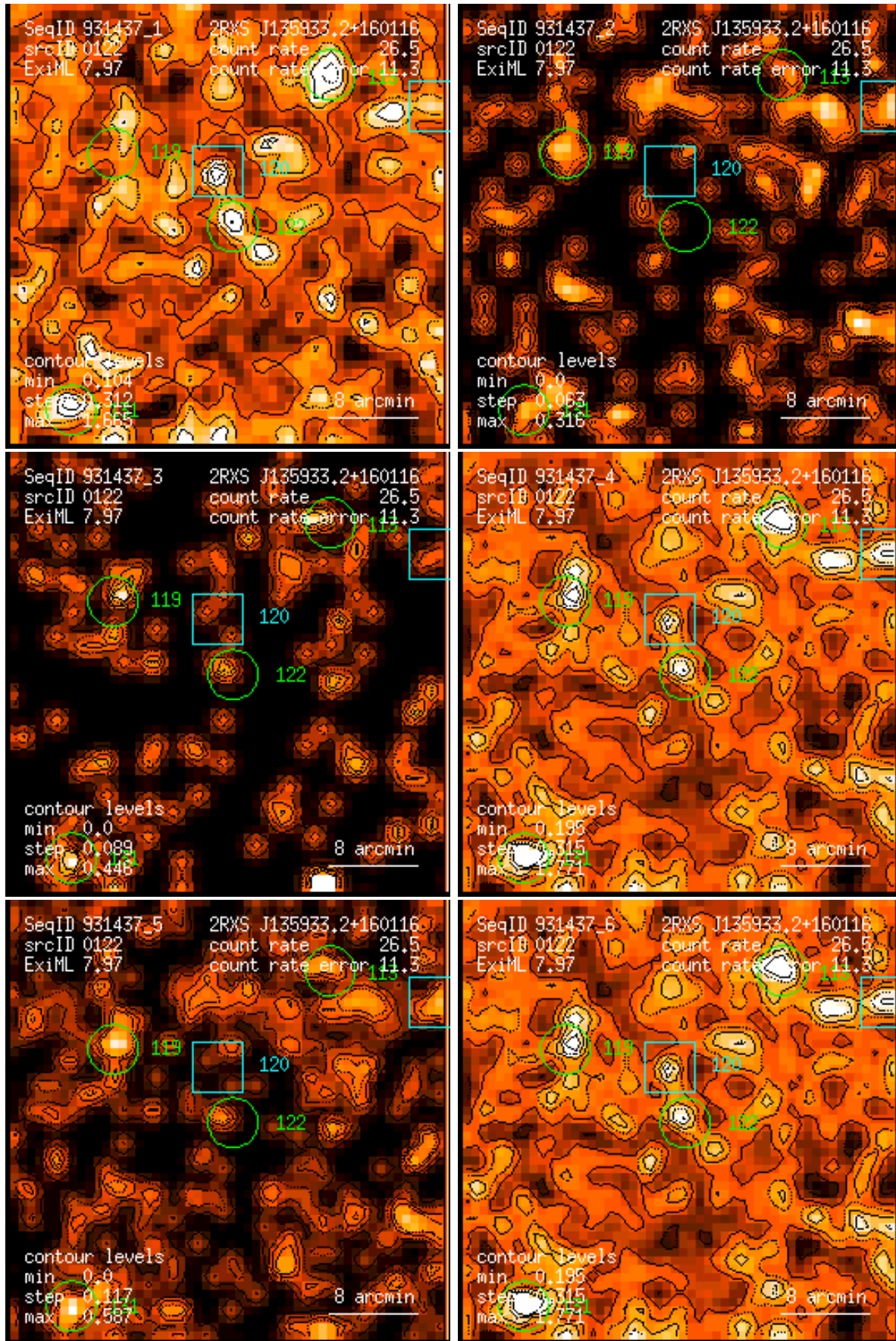
Figure 122: RASS 931437: detection 0122: band rate images, Gaussian filter: (1) PSPC channels 11 – 41, (2) 52 – 90, (3) 91 – 201, (4) 11 – 235, (5) 52 – 201, (6) 11 – 201. Broad band rates in counts/ks. Band rate contour levels in counts/ks/arcmin 2 .
