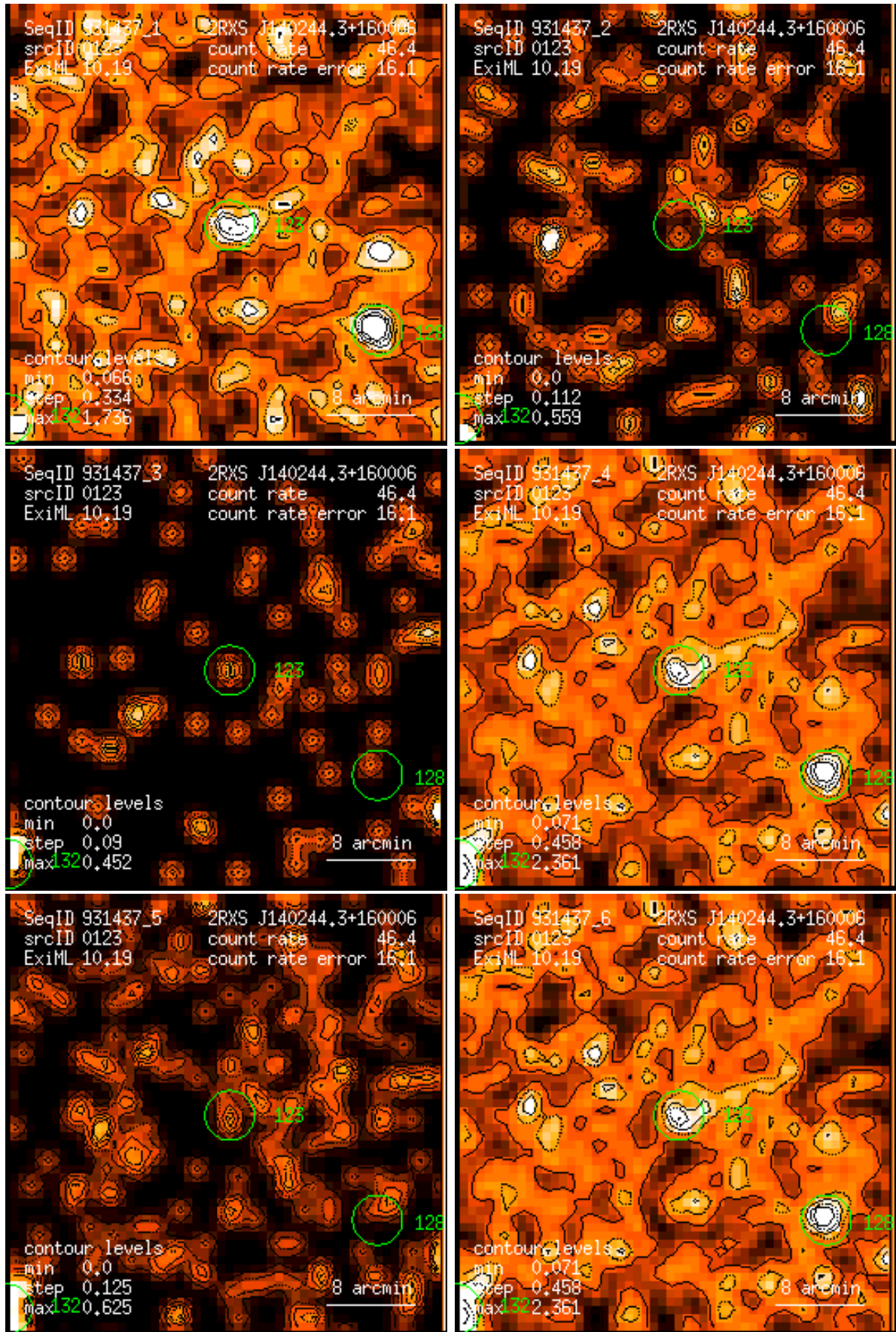
Figure 123: RASS 931437: detection 0123: band rate images, Gaussian filter: (1) PSPC channels 11 – 41, (2) 52 – 90, (3) 91 – 201, (4) 11 – 235, (5) 52 – 201, (6) 11 – 201. Broad band rates in counts/ks. Band rate contour levels in counts/ks/arcmin 2 .
